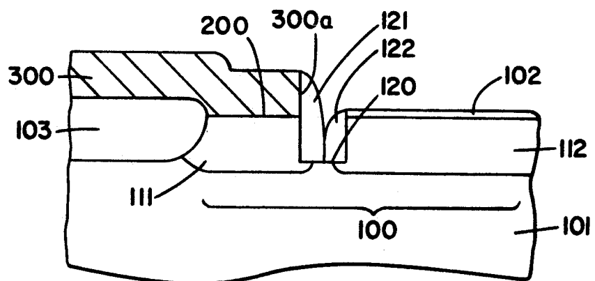
Fig. 3C (PRIOR ART)
