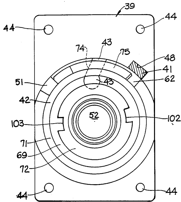
FIG. 5 PRIOR ART
