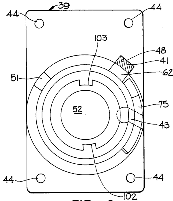
FIG. 6 PRIOR ART
