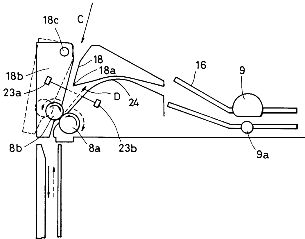
FIG. 13 PRIOR ART
