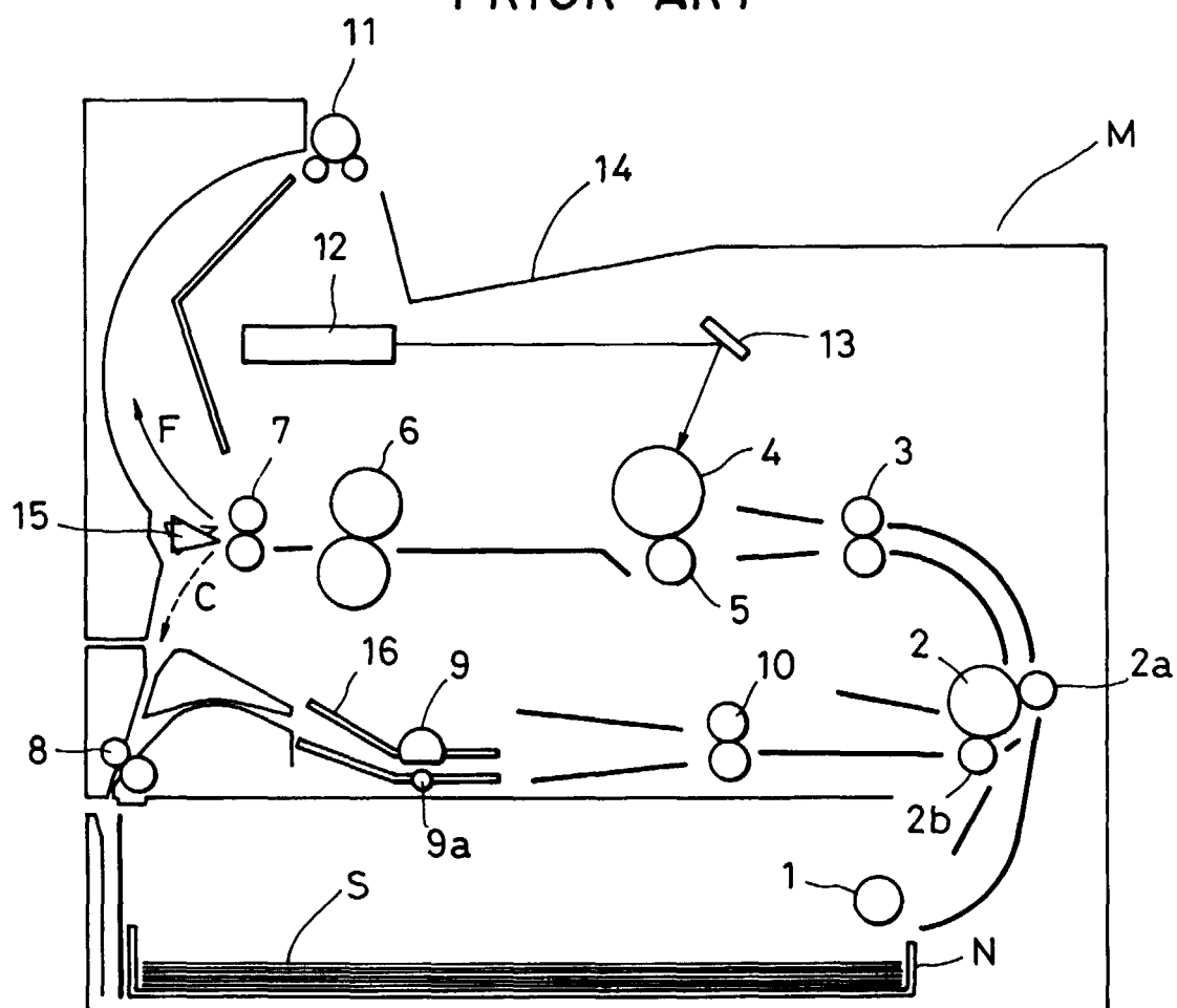
FIG. II PRIOR ART
