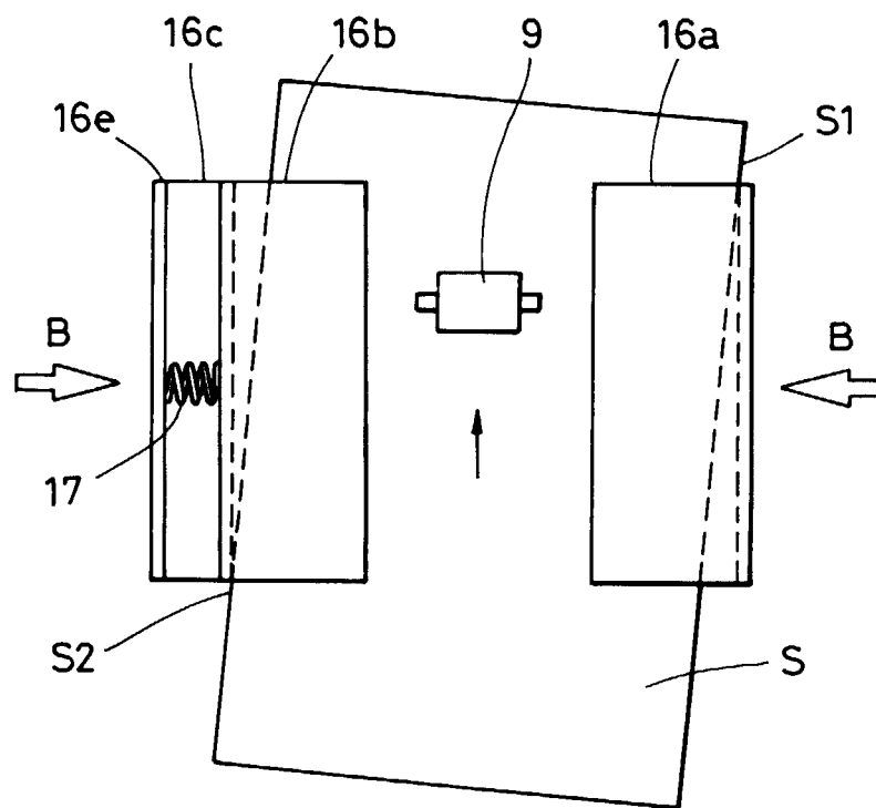
FIG. 14 PRIOR ART
