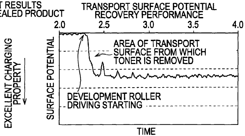
FIG. 9C 400°C ANNEALED PRODUCT
