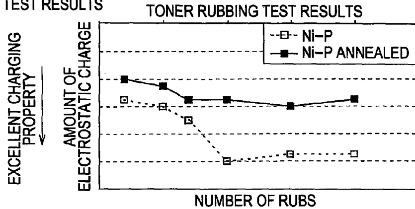
FIG. 9B ACTUAL APPARATUS TEST RESULTS NON-ANNEALED PRODUCT
