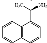
(R)-(+)-1-(1-Naphthyl)ethylamine;
