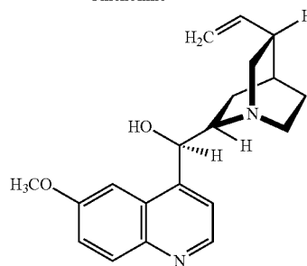
Quinine
