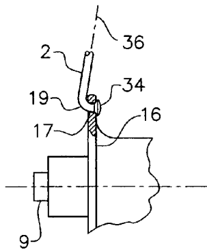
FIG. 2c Prior Art
