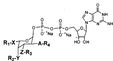
GDP-fucose-derivatives
