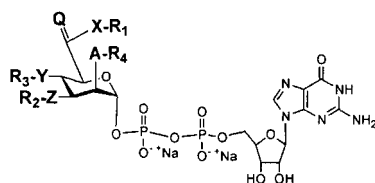
GDP-Mannose-derivatives
