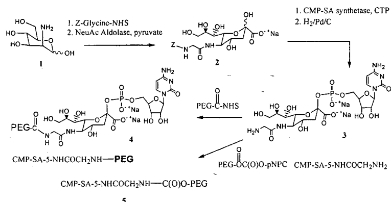
Scheme 4
