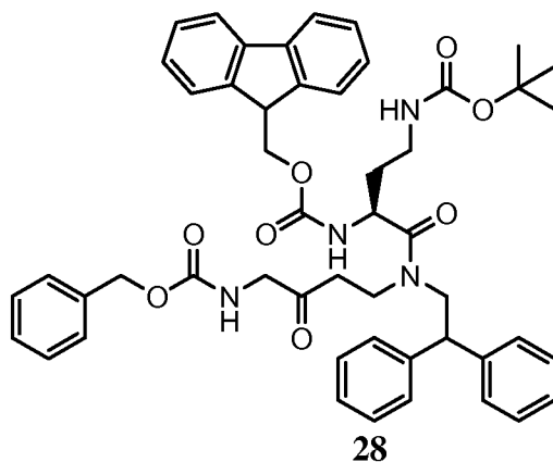
28 (S)-9-fluorenylmethyl 10-(2,2-diphenylethyl)-2,2-dimethyl-18-phenyl-4,9,13,16-tetraoxo-3,17-dioxa-5,10,15-triazaoctadecan-8-ylcarbamate
