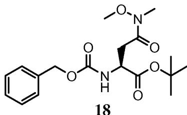
18 ( S )-tert-butyl 3-methyl-4,8-dioxo-10-phenyl-2,9-dioxa-3,7-diazadecane-6-carboxylate
