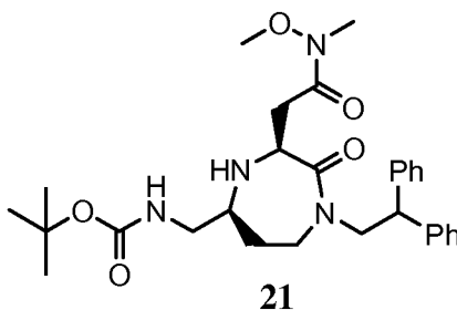
tert -butyl ((3 S ,5 S )-1-(2,2-diphenylethyl)-3-(2-(methoxy(methyl)amino)-2-oxoethyl)-2-oxo-1,4-diazepan-5-yl)methylcarbamate
