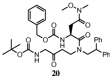
( S )-benzyl 8-(2,2-diphenylethyl)-3,16,16-trimethyl-4,7,11,14-tetraoxo-2,15-dioxo-3,8,13-triazaheptadecan-6-ylcarbamate
