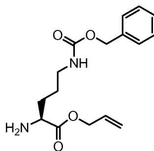
90 (S)-allyl 2-amino-5-(benzyloxycarbonylamino)pentanoate
