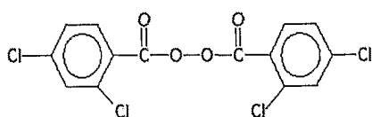
dichlorobenzoyl peroxide
