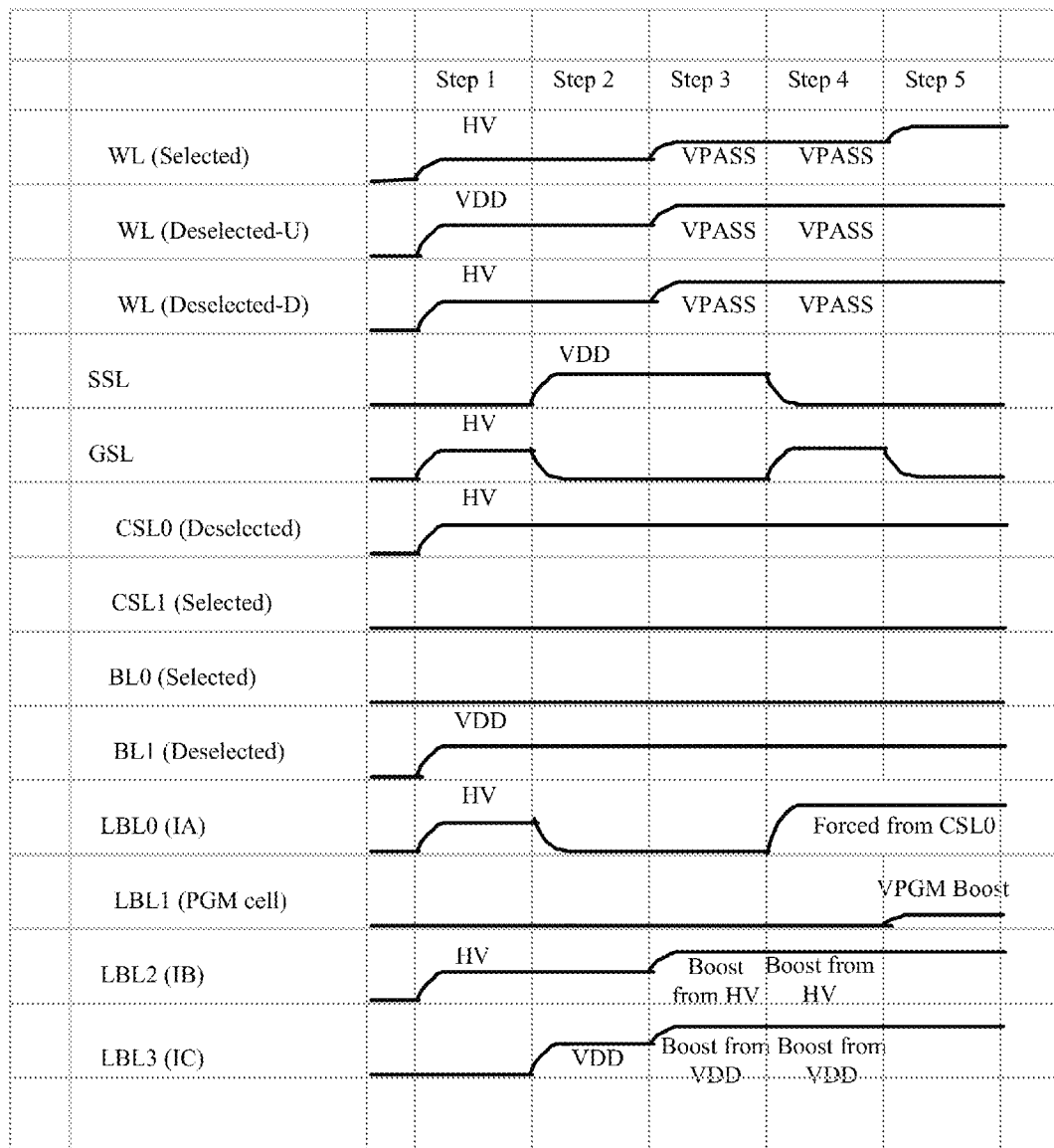
SL SIDE DIODE 1ST PROGRAM SEQUENCE
