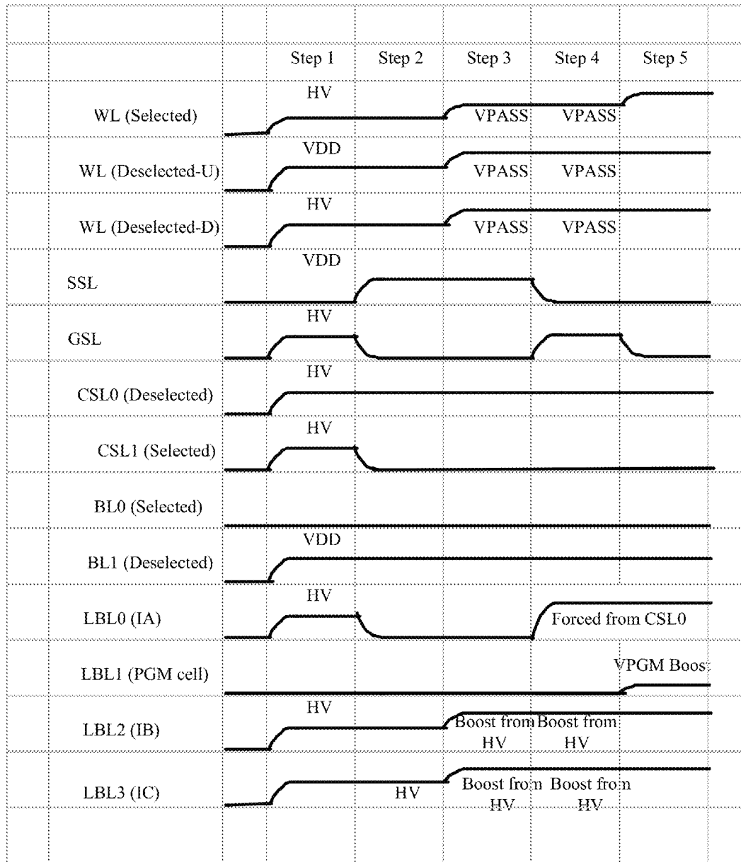
SL SIDE DIODE 2ND PROGRAM SEQUENCE
