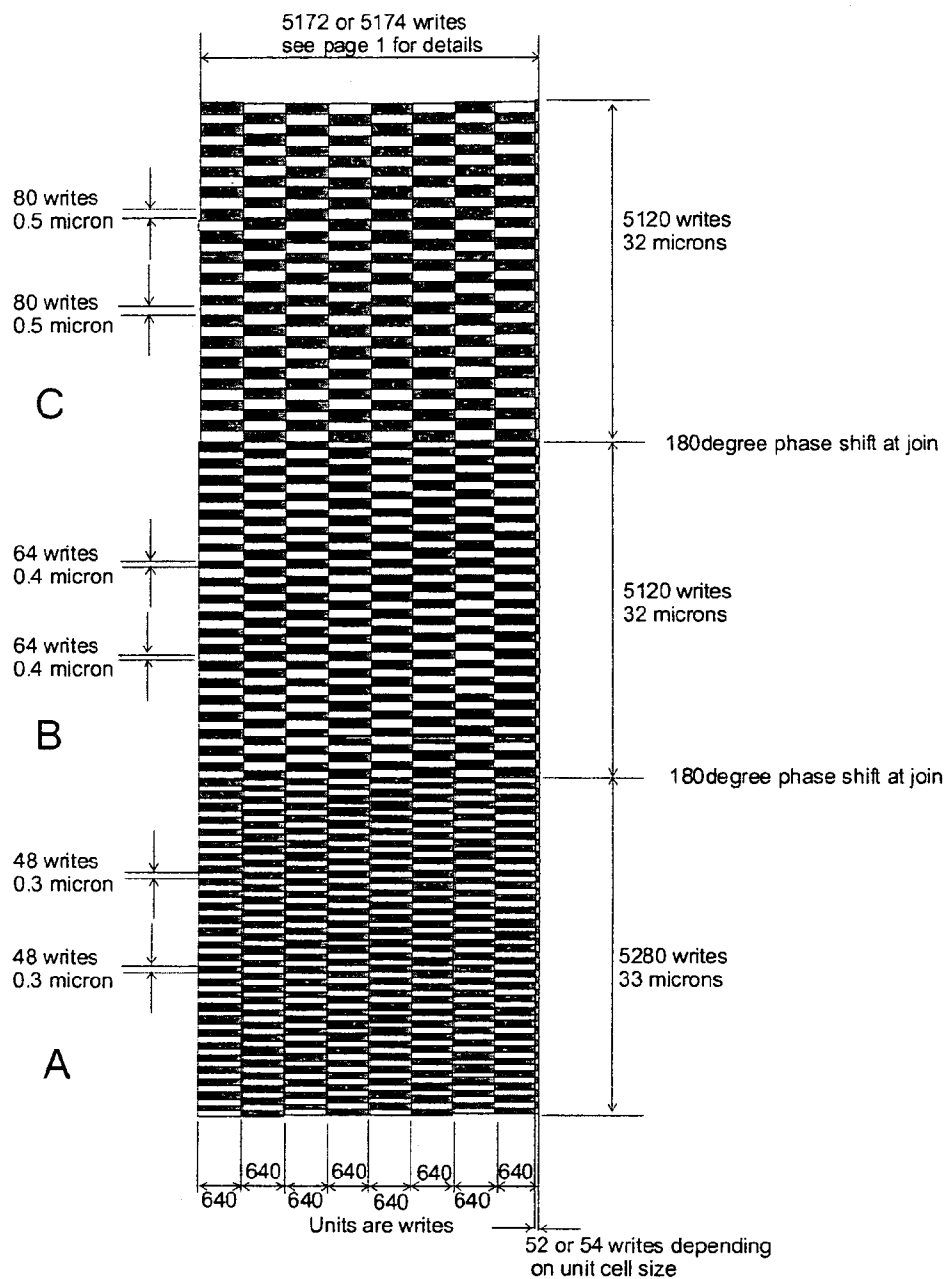
FIGURE 21 Example of grating design with areas of different pitch, and incorporating slips according to the present invention.
