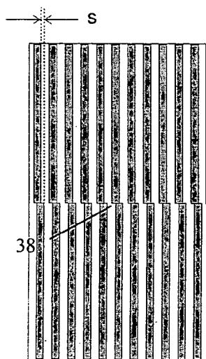
Fig. 8c Slip plane (phase = 2\pi.s/p )
