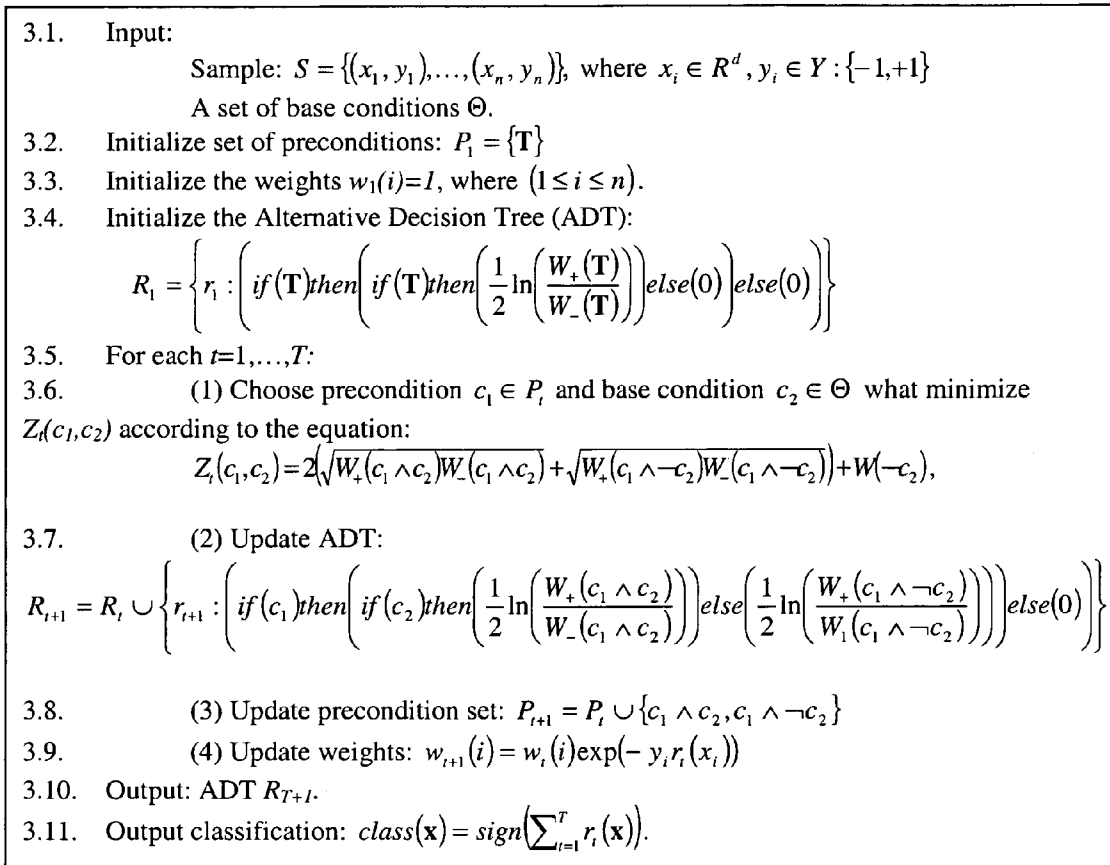
FIG. 3: Boosting Alternating Decision Tree
