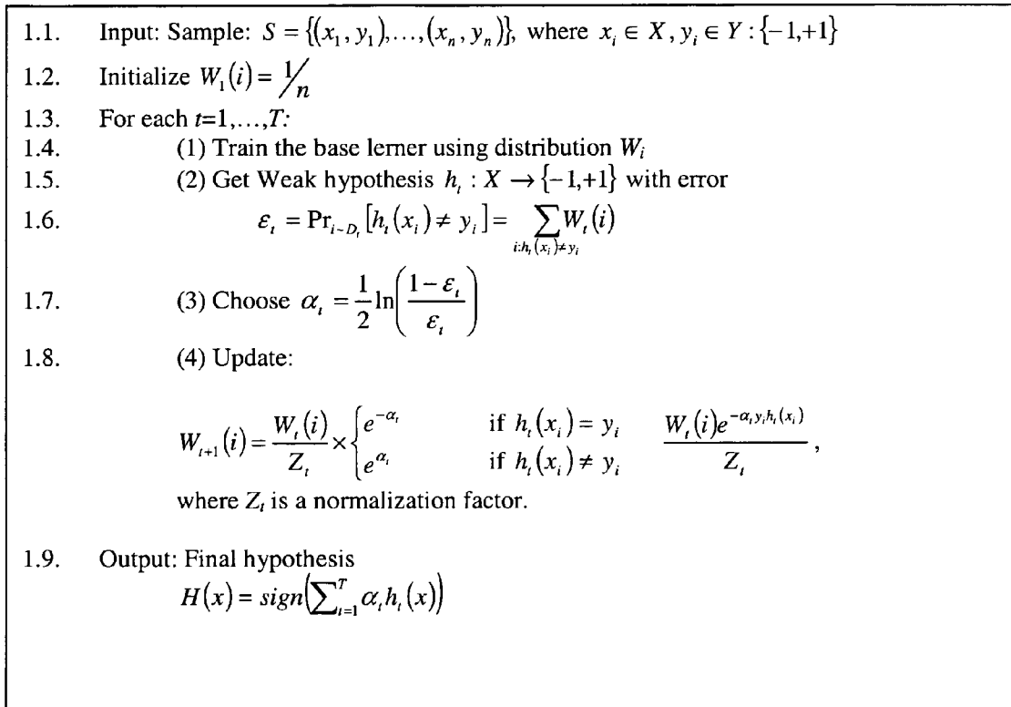
FIG. 1: The AdaBoost Algorithm
