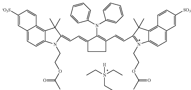
[Chemical Formula 21]
