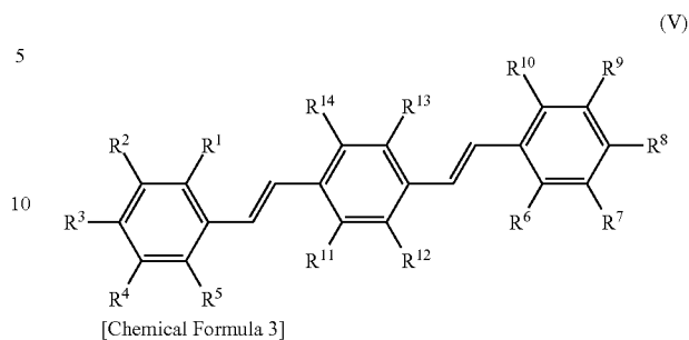
[Chemical Formula 3]
