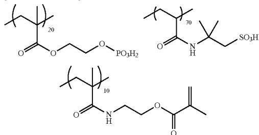
[Chemical Formula 20]
