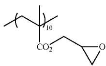
[Chemical Formula 10]
