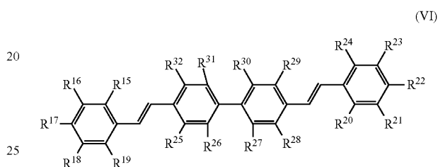
[Chemical Formula 3]
