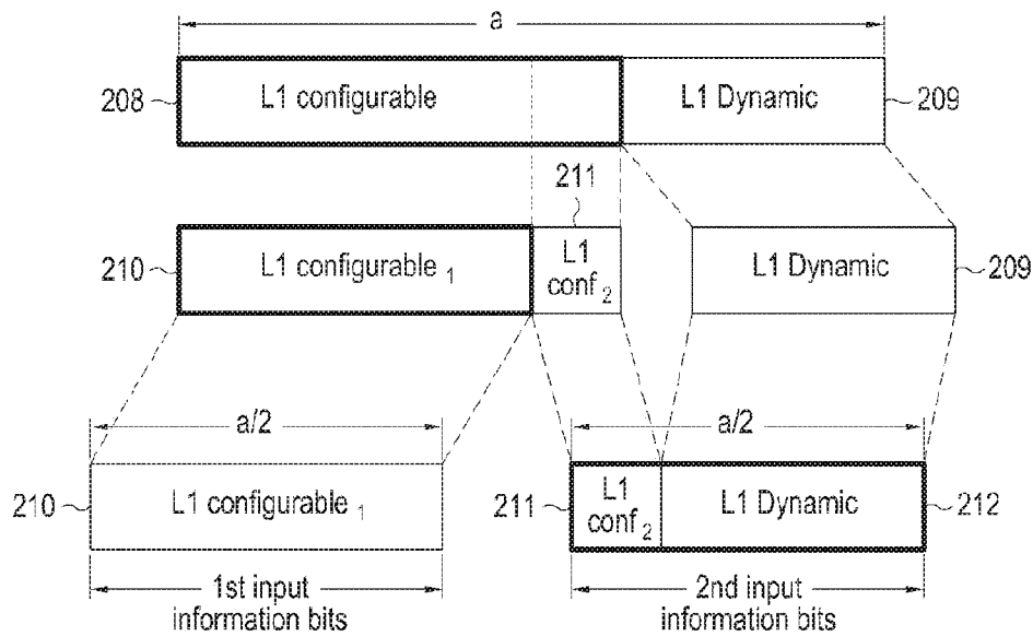
FIG. 2 (PRIOR ART)
