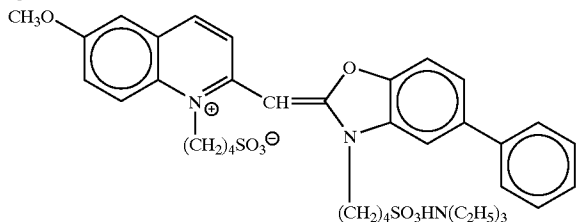
Spectral sensitizer 7
