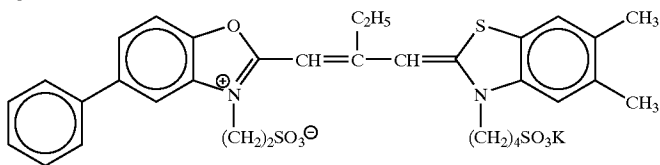
Spectral sensitizer 7
