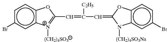
Spectral sensitizer 5
