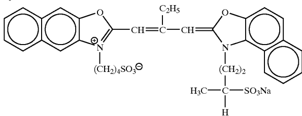
Spectral sensitizer 6
