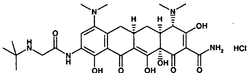
Figure A: Chemical structure of Tigecycline hydrochloride
