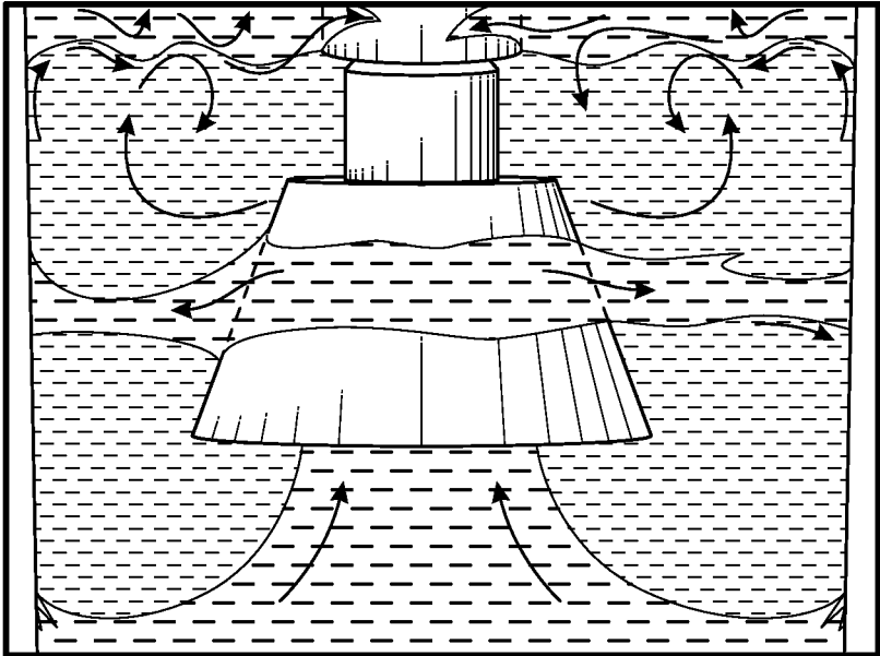
FIG. 6 (PRIOR ART)
