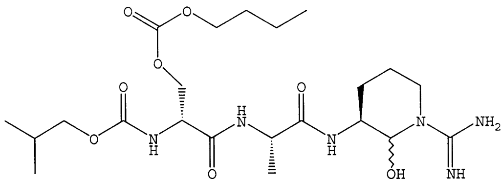
isobutoxycarbonyl-D- (n-butyloxycarbonyl) -Ser-L-Ala-argininal;
