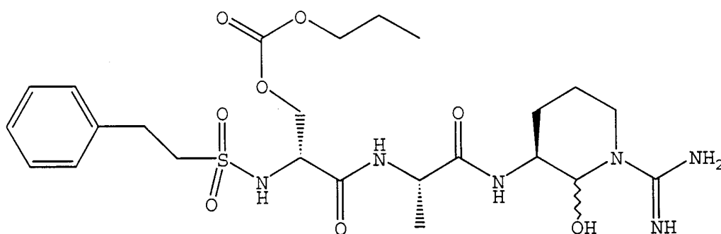
phenethylsulfonyl-D-(n-propyloxycarbonyl)-Ser-L-Ala-argininal;
