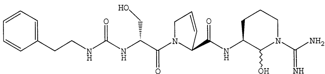
3-phenethylaminocarbonyl-D-Ser-L-dehydroprolyl-argininal;
