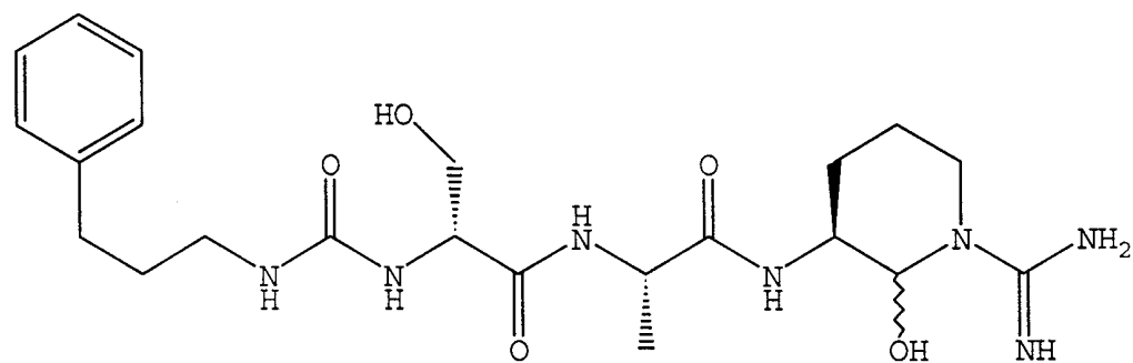
3-phenpropylaminocarbonyl-D-Ser-L-Ala-argininal;
