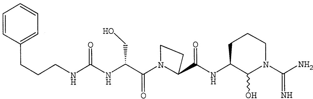
3-phenpropylaminocarbonyl-D-Ser-L-azetidine-2-carboxy-argininal;
