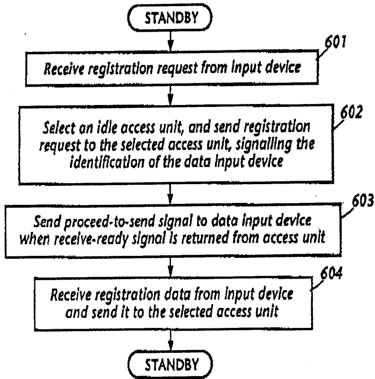
FIG. 6 MAIN UNIT (REGISTRATION MODE)
