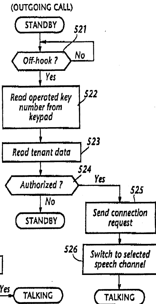
FIG. 5B CORDLESS STATION (OUTGOING CALL)
