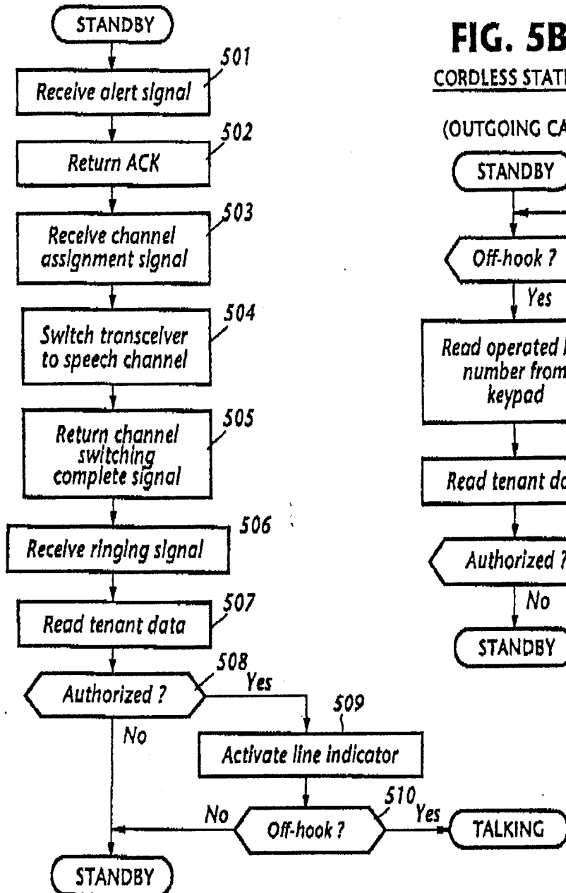
FIG. 5A CORDLESS STATION (INCOMING CALL)
