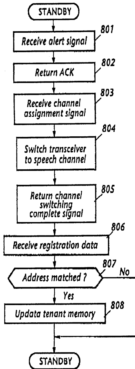
FIG. 8 CORDLESS STATION (REGISTRATION MODE)
