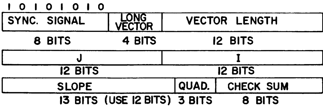
FIG _ 4 LONG VECTOR MESSAGE
