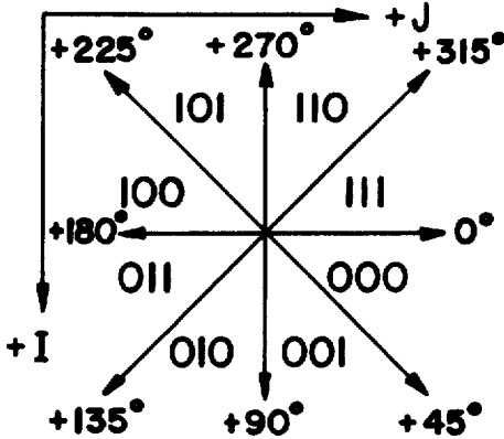
FIG _ 4 LONG VECTOR MESSAGE
