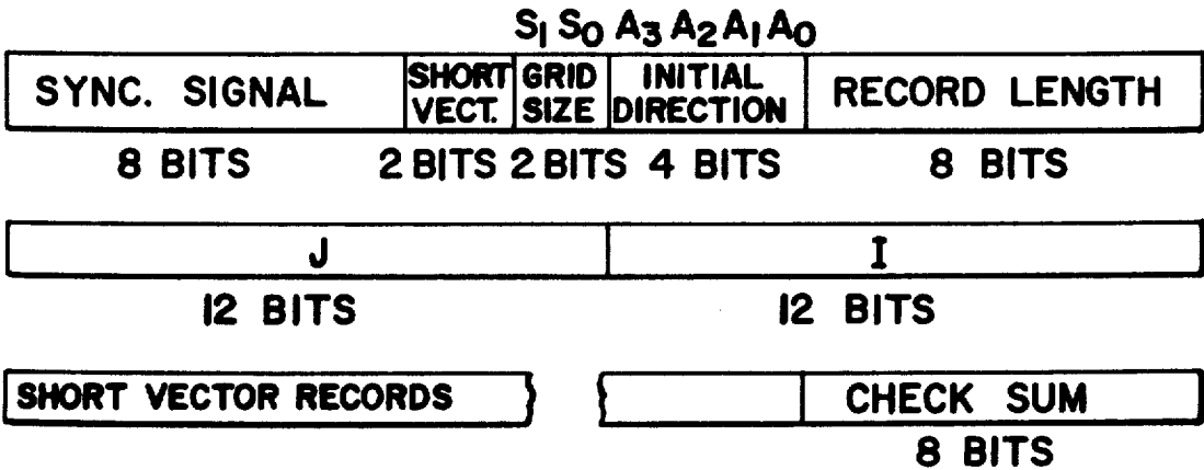
SHORT VECTOR MESSAGE
