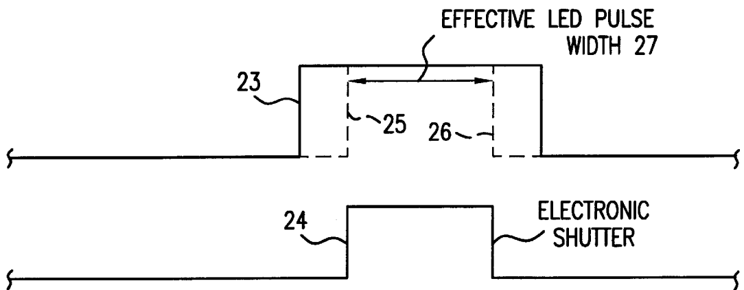
FIG.4 (GATE LIGHT WITH SHUTTER)
