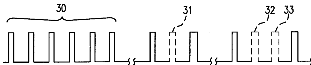
FIG.6 (SUPPRESSED CYCLE SAMPLING)
