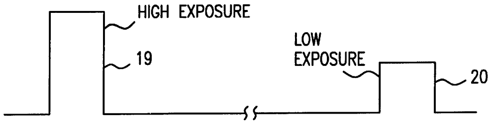
FIG.2 (LED PULSE AMPLITUDE)
