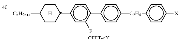
CFET-nX
