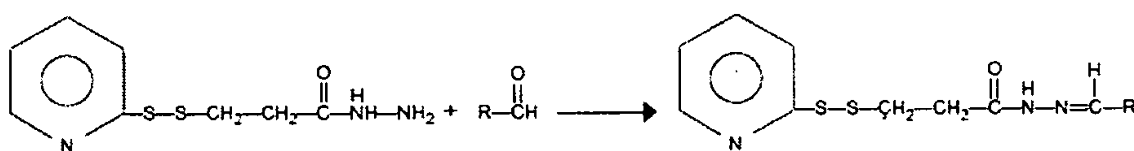
PDP Hydrazide 3-(2-pyridyldithio)propionyl Hydrazide MW 229.31
