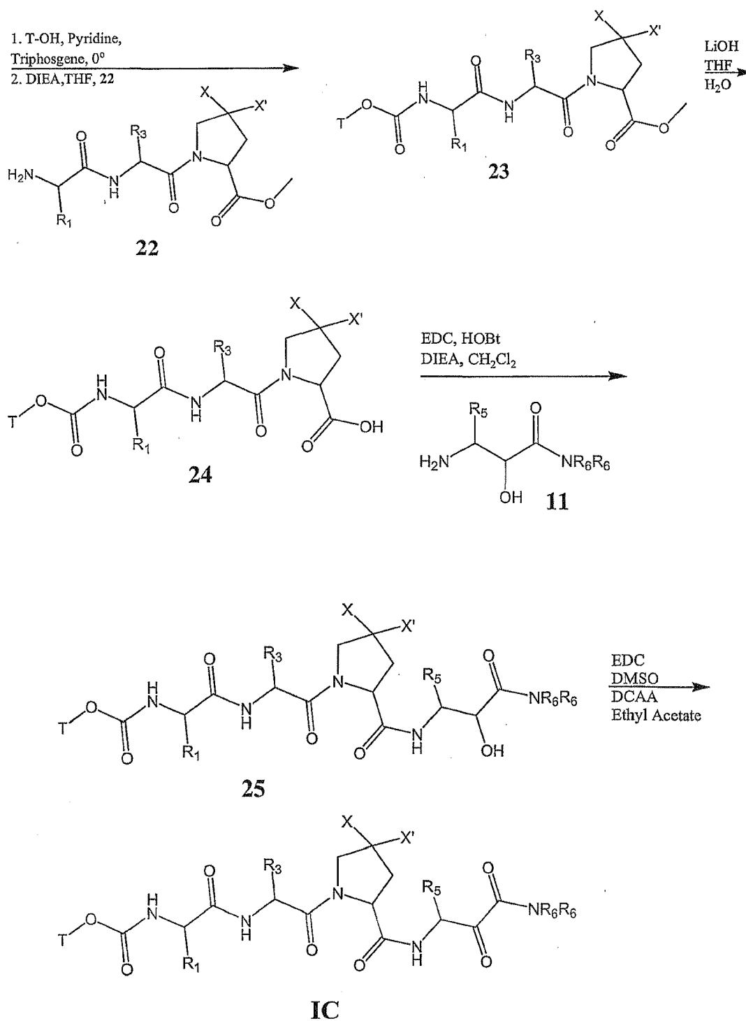
Scheme 3:
