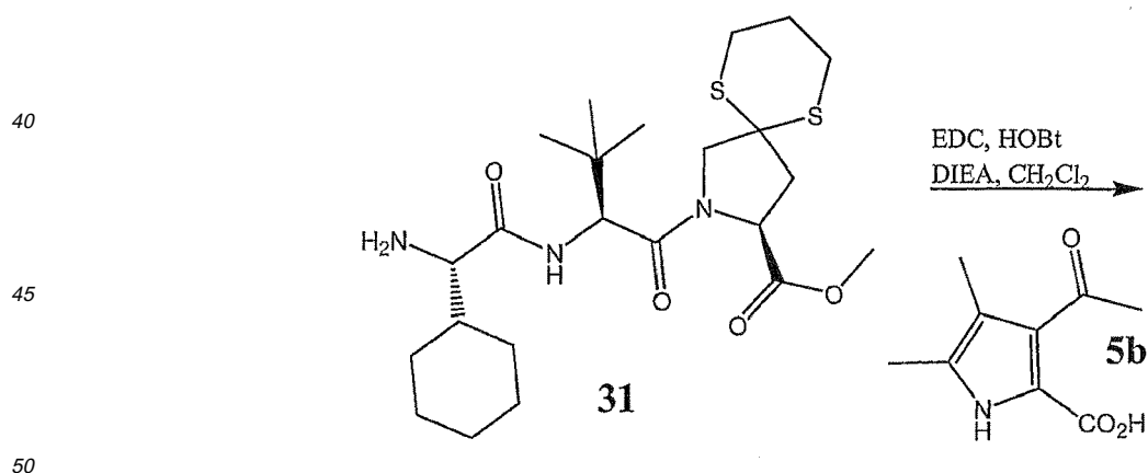
35 Scheme 6:
