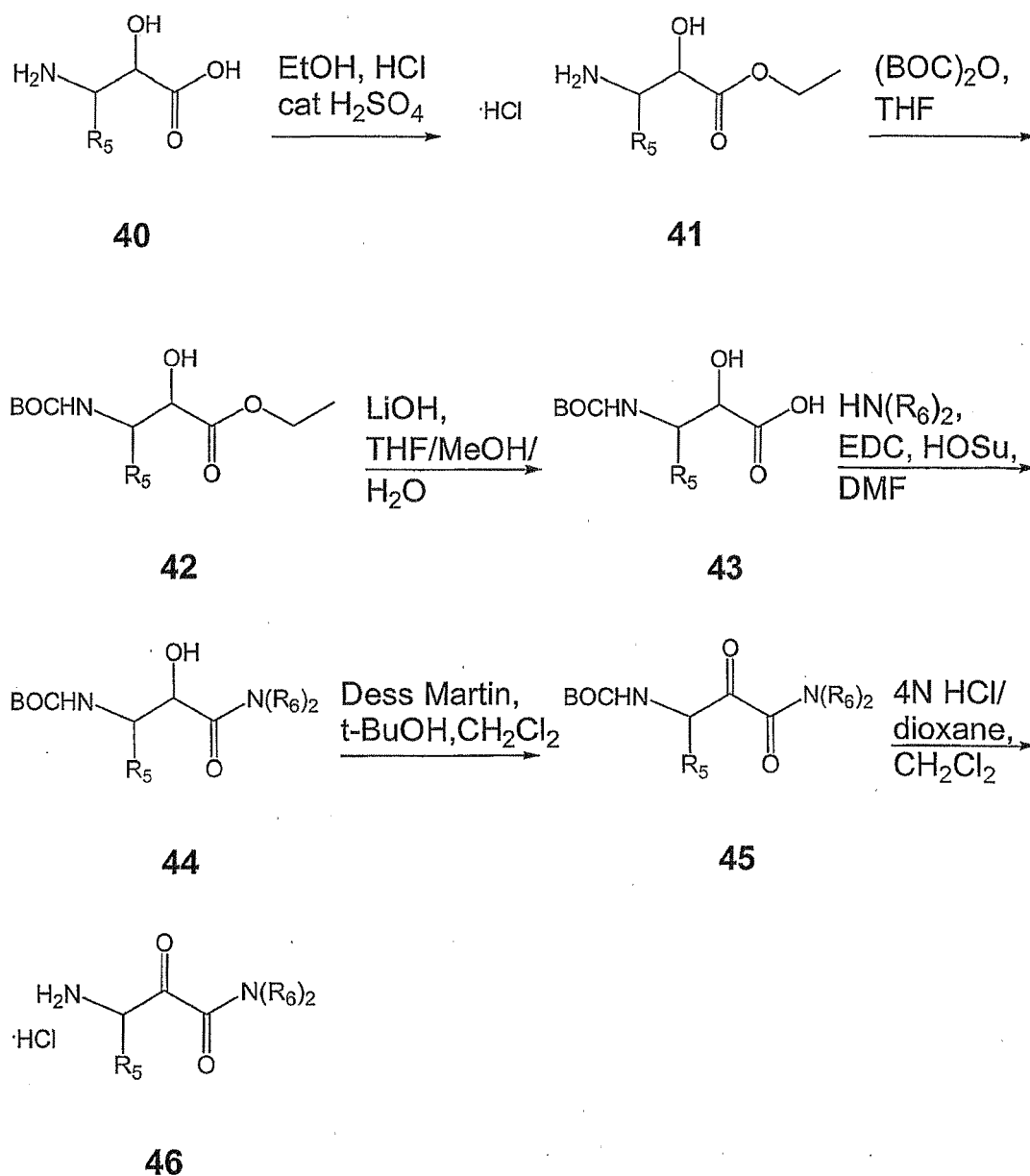
Scheme 1A:
