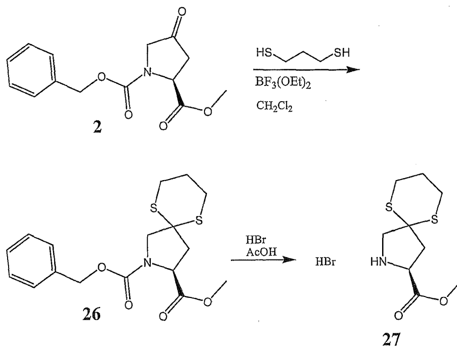
Scheme 5:
