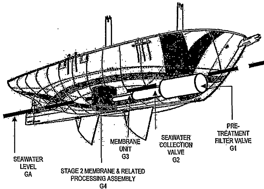
Figure 3 illustrates filtered seawater incoming from the valve fitted onto the hull of the sea vessel, being routed onto a assembly of devlces capable of performing reverse osmosis to further purify the filtered seawater
