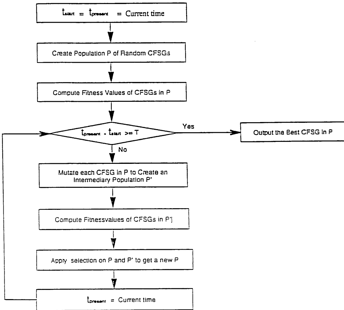
Evolutionary algorithms based optimization technique.
