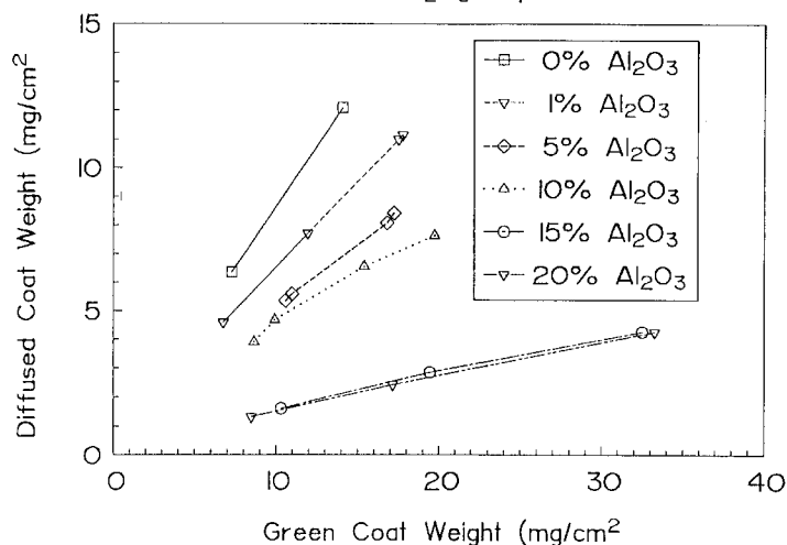
Green vs Diffused Coat Weight for 0-20% Al 2 O 3 Doped PtAlSi
