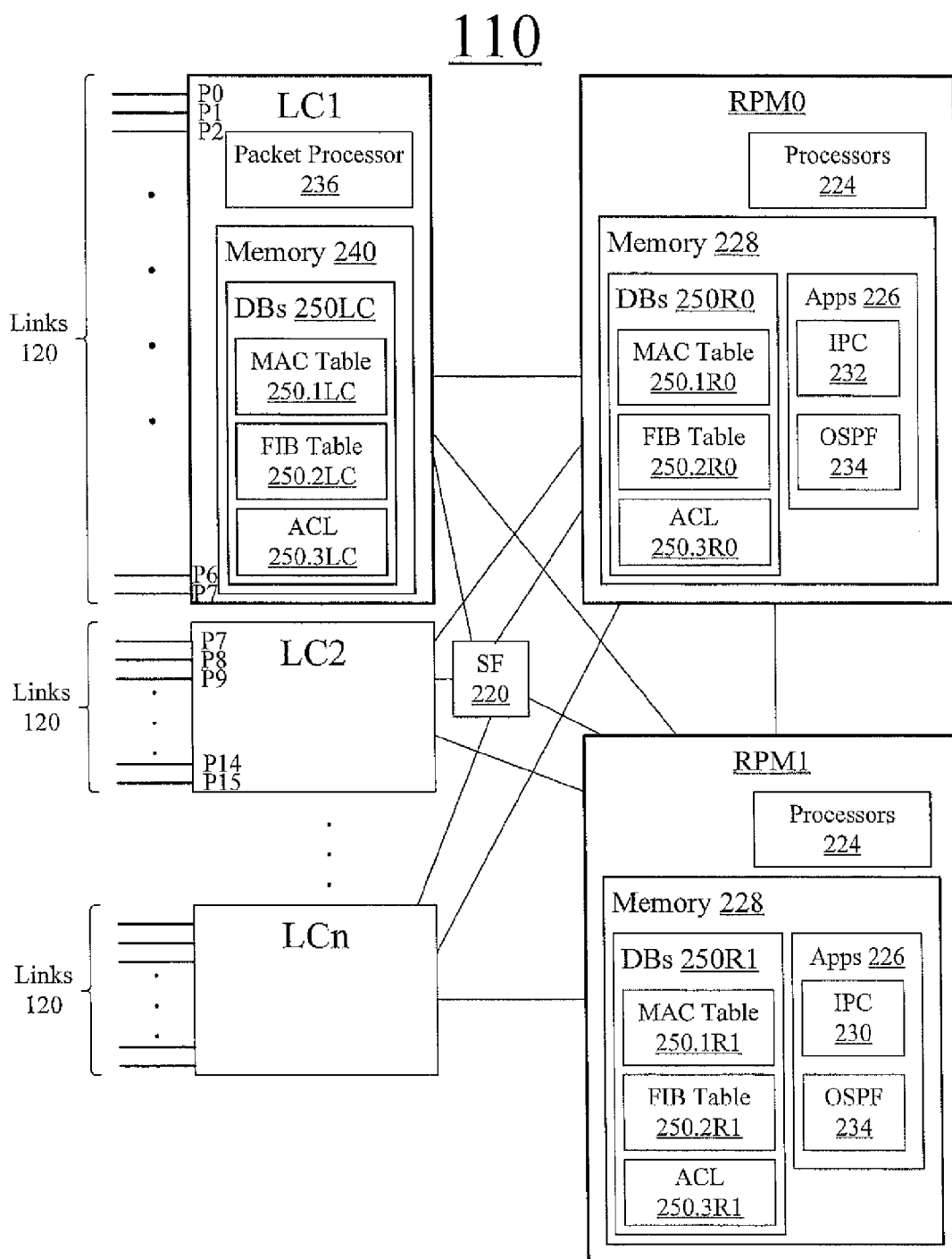
FIG. 2 PRIOR ART
