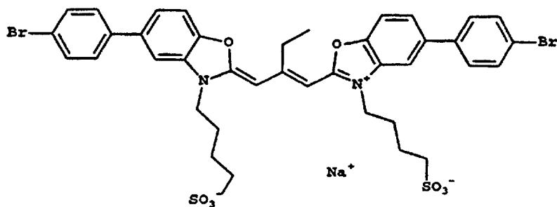
Dye 8
