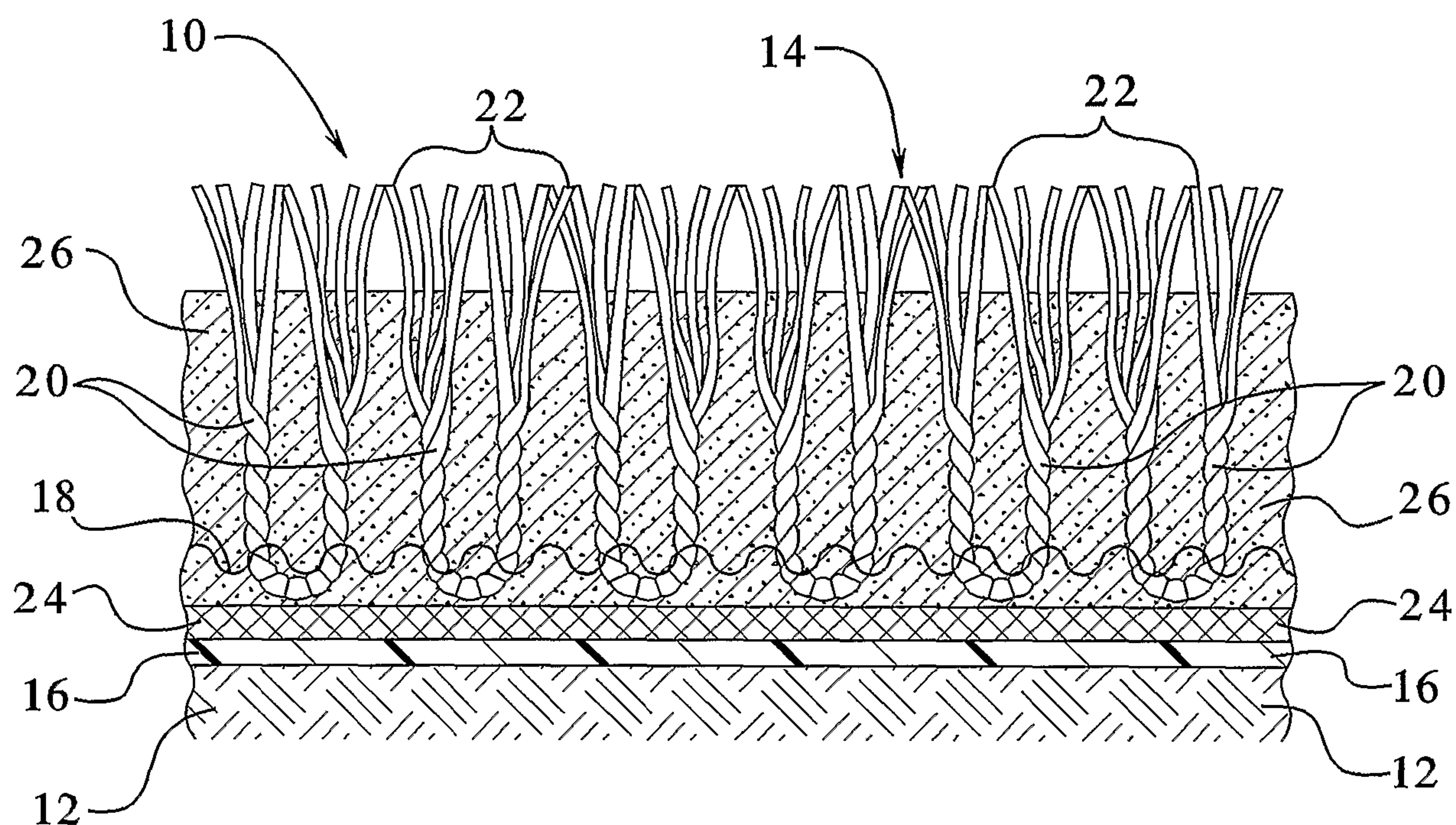
FIG.1 (PRIOR ART)
