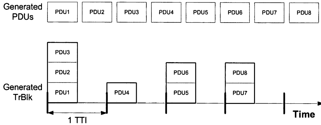
Figure 7 - Transport Channel Block generation
