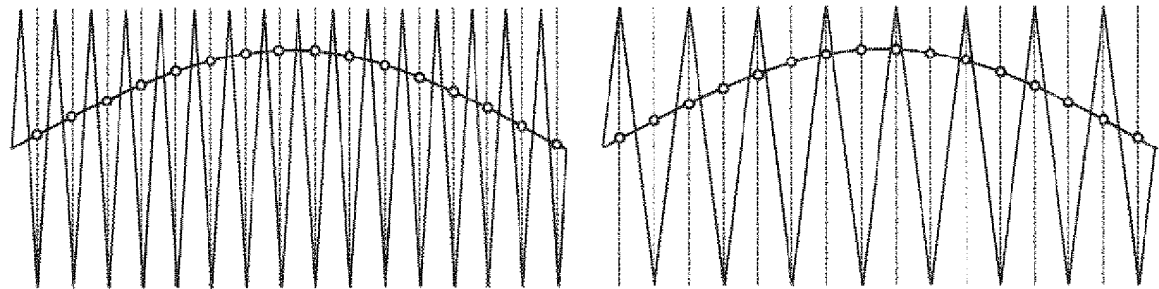
CONTROL FREQUENCY * 2 > CARRIER FREQUENCY ( fc2 ) CONTROL FREQUENCY * 2 ≤ CARRIER FREQUENCY ( fc1 )
