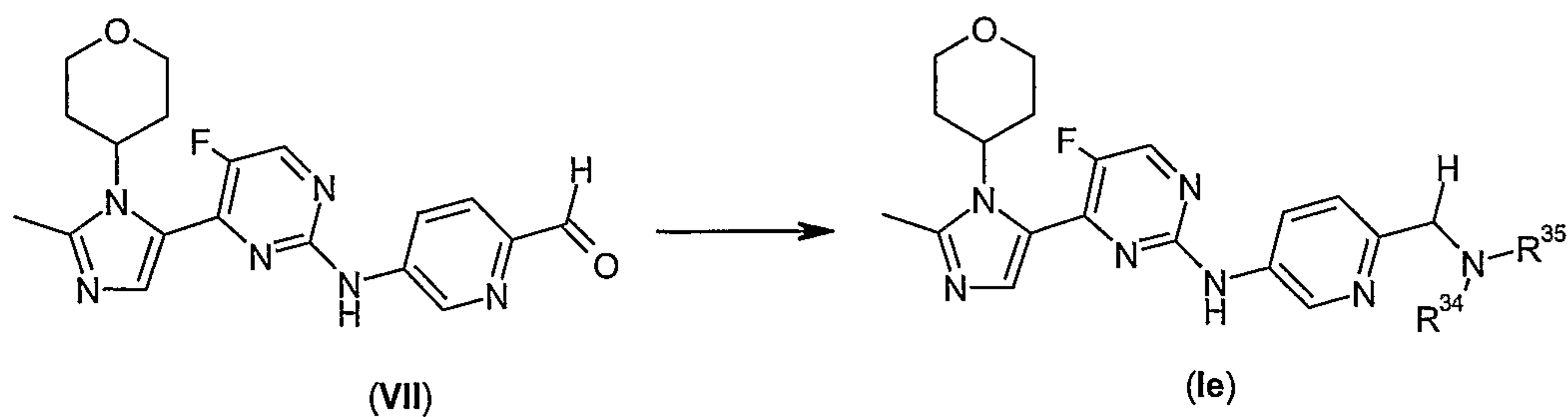
Scheme 6
