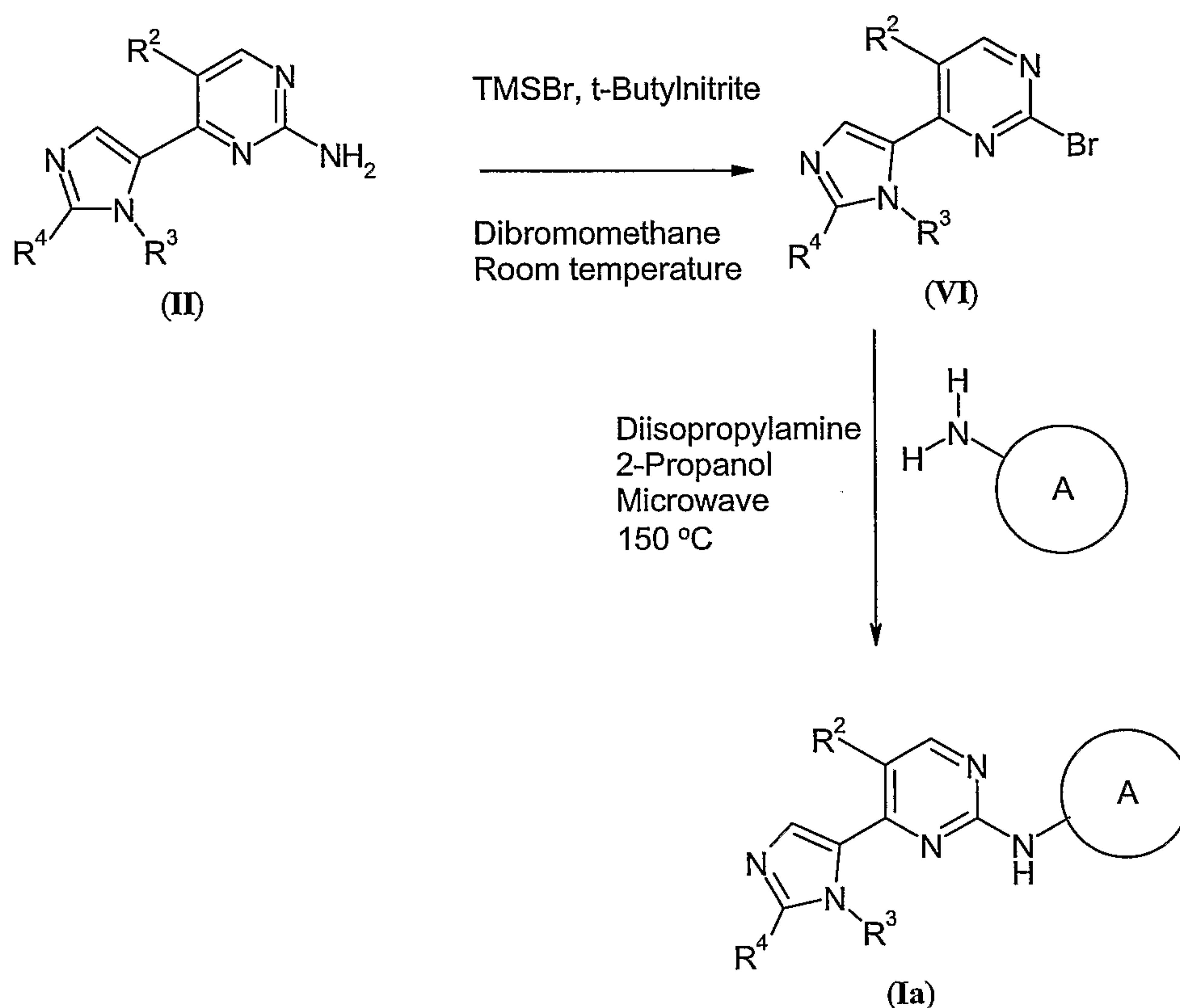
Scheme 4
