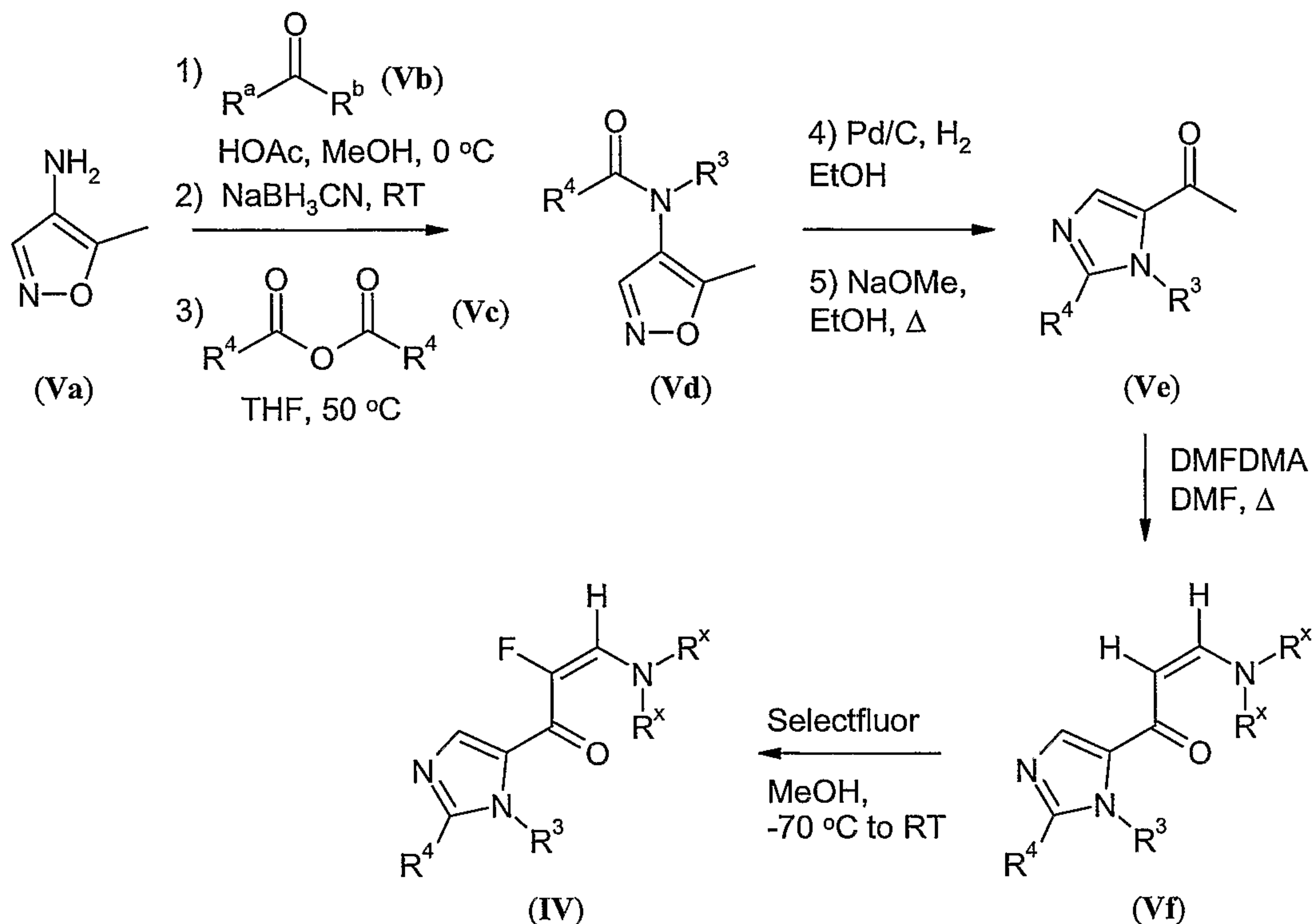
Scheme 3
