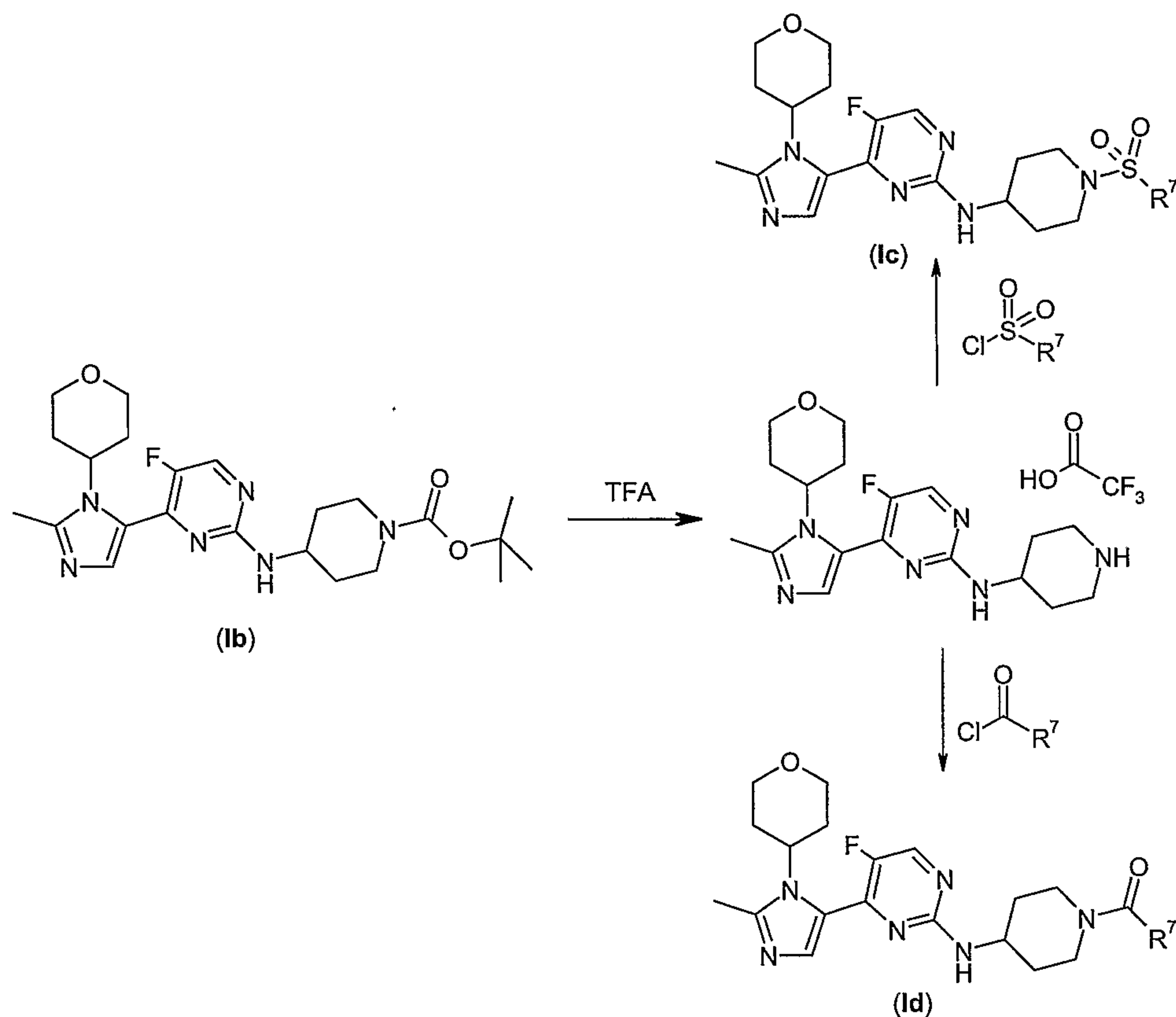
Scheme 5
