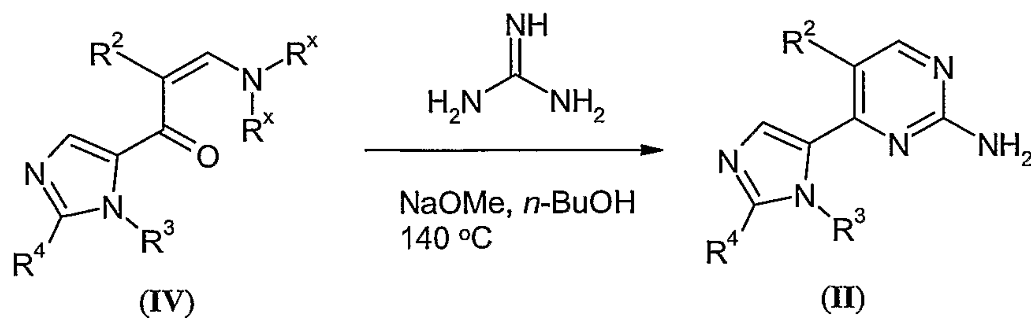
Scheme 2
