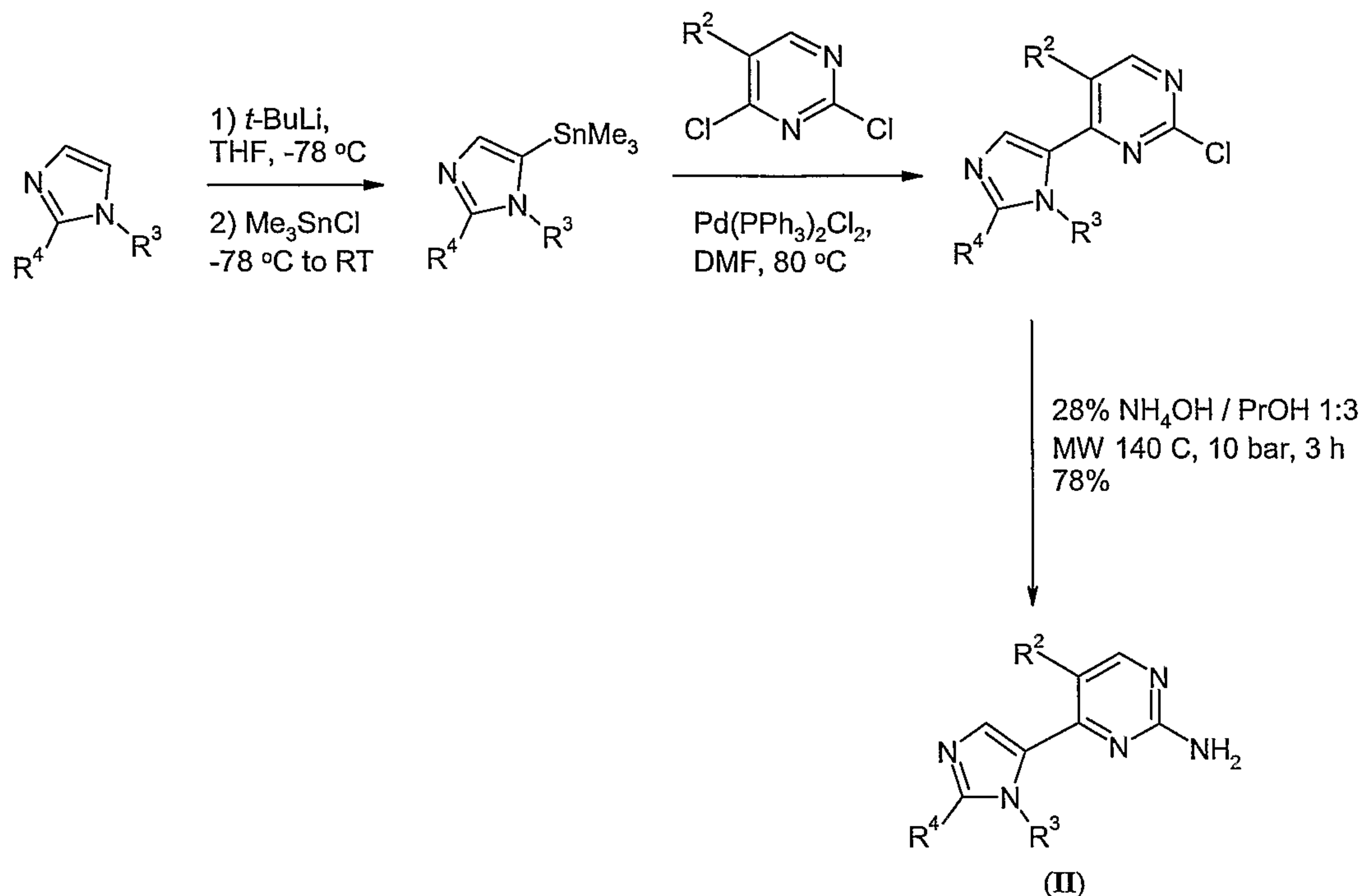
Scheme 1
