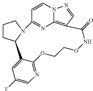
(6R)-9-fluoro-13,16-dioxo-2,11,17,21,22,25-hexaazapentacyclo[17.5.2.0 2,6 .0 7,12 .0 22,26 ]hexacos-1(25),7,9,11,19(26),20,23-heptaen-18-one
