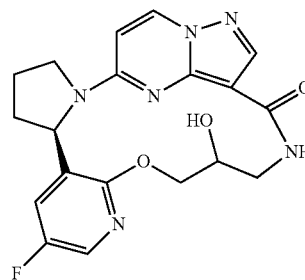
(6R)-9-fluoro-15-hydroxy-13-oxa-2,11,17,21,22,25-hexaazapentacyclo[17.5.2.0 2,6 .0 7,12 .0 22,26 ]hexacos-1(25),7,9,11,19(26),20,23-heptaen-18-one
