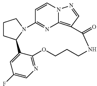
(6R)-9-fluoro-13-oxa-2,11,17,21,22,25-hexaazapentacyclo[17.5.2.0 2,6 .0 7,12 .0 22,26 ]hexacos-1(25),7,9,11,19(26),20,23-heptaen-18-one
