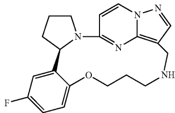
(6R)-9-fluoro-13-oxa-2,17,21,22,25-pentaazapentacyclo[17.5.2.0 2,6 .0 7,12 .0 22,26 ]]hexacos-1(25),7,9,11,19(26),20,23-heptaene
