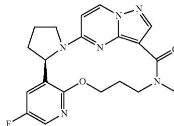
(6R)-9-fluoro-17-methyl-13-oxa-2,11,17,21,22,25-hexaazapentacyclo[17.5.2.0 2,6 .0 7,12 .0 22,26 ]hexacos-1(25),7,9,11,19(26),20,23-heptaen-18-one
