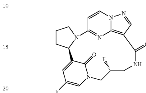
(6R,13R)-9,13-difluoro-2,11,15,19,20,23-hexaazapentacyclo[15.5.2.1 7,11 .0 2,6 .0 20,24 ]pentacos-1(23),7,9,17(24),18,21-hexaene-16,25-dione
