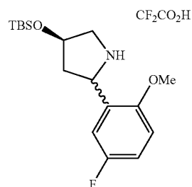
(R)-4-((tert-butyldimethylsilyl)oxy)-2-(5-fluoro-2-methoxyphenyl)pyrrolidine 2,2,2-trifluoroacetate
