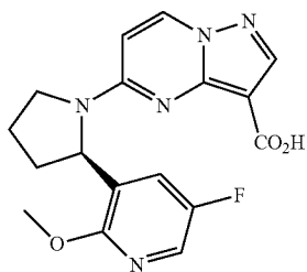
(R)-5-(2-(5-fluoro-2-methoxypyridin-3-yl)pyrrolidin-1-yl)pyrazolo[1,5-a]pyrimidine-3-carboxylic acid
