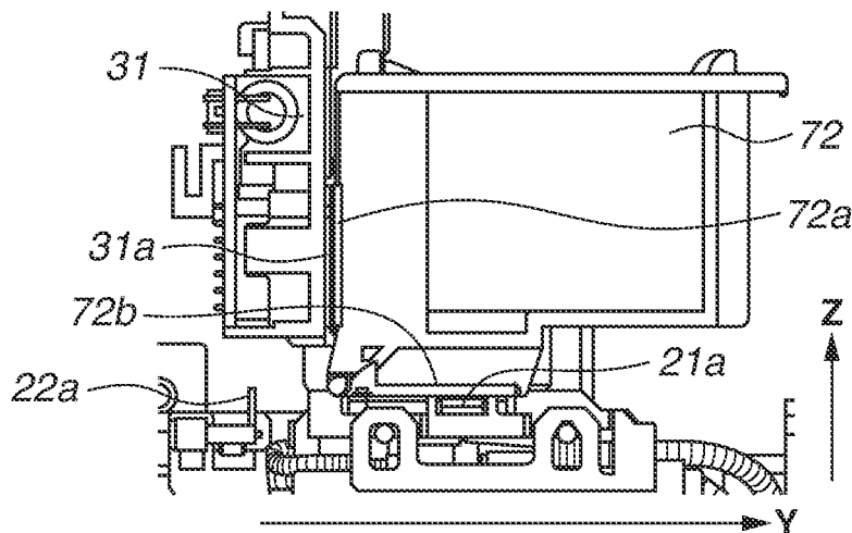
SIDE VIEW IN CAPPING STATE
