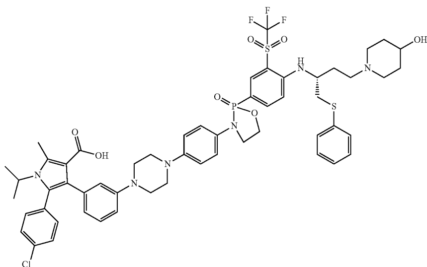
5-(4-chlorophenyl)-4-(3-(4-(4-(2-(4-((R)-4-(4-hydroxypiperidin-1-yl)-1-(phenylthio)butan-2-yl)amino-3-((trifluoromethyl)sulfonyl)phenyl)-2-oxido-1,3,2-oxazaphospholidin-3-yl)phenyl)piperazin-1-yl)phenyl)-1-isopropyl-2-methyl-1H-pyrrole-3-carboxylic acid
