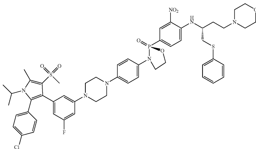
(S)-3-(4-(4-(3-(2-(4-chlorophenyl)-1-isopropyl-5-methyl-4-(methylsulfonyl)-1H-pyrrol-3-yl)-5-fluorophenyl)piperazin-1-yl)phenyl)-2-(4-(((R)-4-morpholino-1-(phenylthio)butan-2-yl)amino)-3-nitrophenyl)-1,3,2-oxazaphospholidine 2-oxide
