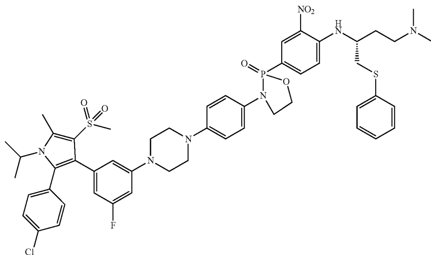
3-(4-(4-(3-(2-(4-chlorophenyl)-1-isopropyl-5-methyl-4-(methylsulfonyl)-1H-pyrrol-3-yl)-5-fluorophenyl)piperazin-1-yl)phenyl)-2-(4-((R)-4-(dimethylamino)-1-(phenylthio)butan-2-yl)amino)-3-nitrophenyl)-1,3,2-oxazaphospholidine 2-oxide
