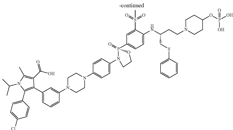
5-(4-chlorophenyl)-1-isopropyl-2-methyl-4-(3-(4-(4-((R)-2-(3-(methylsulfonyl)-4-((R)-1-(phenylthio)-4-(4-(phosphonoxy)piperidin-1-yl)butan-2-yl)amino)phenyl)-2-oxido-1,3,2-oxazaphospholidin-3-yl)phenyl)piperazin-1-yl)phenyl)-1H-pyrrole-3-carboxylic acid
