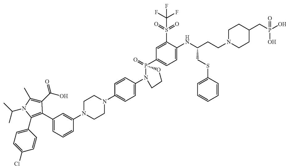
5-(4-chlorophenyl)-1-isopropyl-2-methyl-4-(3-(4-(4-((R)-2-oxido-2-(4-(((R)-1-(phenylthio)-4-(4-(phosphonomethyl)piperidin-1-yl)butan-2-yl)amino)-3-(trifluoromethyl)sulfonyl)phenyl)-1,3,2-oxazaphospholidin-3-yl)phenyl)piperazin-1-yl)phenyl)-1H-pyrrole-3-carboxylic acid
