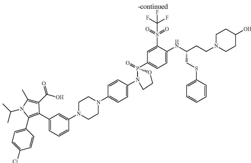
5-(4-chlorophenyl)-4-(3-(4-(4-((R)-2-(4-((R)-4-((R)-4-(4-hydroxypiperidin-1-yl)-1-(phenylthio)butan-2-yl)amino)-3-((trifluoromethyl)sulfonyl)phenyl)-2-oxido-1,3,2-oxazaphospholidin-3-yl)phenyl)piperazin-1-yl)phenyl)-1-isopropyl-2-methyl-1H-pyrrole-3-carboxylic acid
