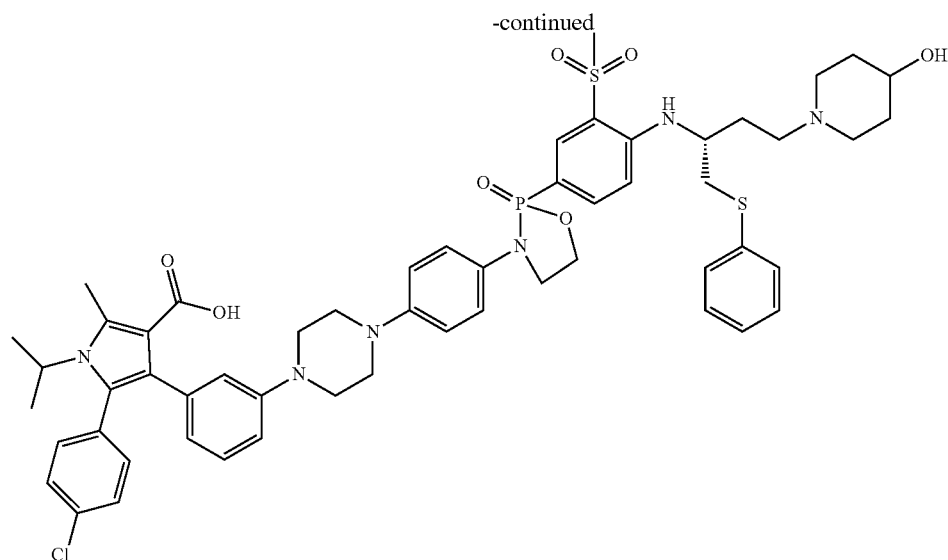
5-(4-chlorophenyl)-4-(3-(4-(4-(2-(4-((R)-4-(4-hydroxypiperidin-1-yl)-1-(phenylthio)butan-2-yl)amino)-3-(methylsulfonyl)phenyl)-2-oxido-1,3,2-oxazaphospholidin-3-yl)phenyl)piperazin-1-yl)phenyl)-1-isopropyl-2-methyl-1H-pyrrole-3-carboxylic acid
