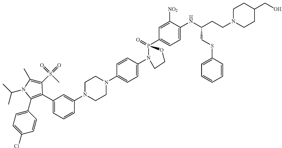
(S)-3-(4-(4-(3-(2-(4-chlorophenyl)-1-isopropyl-5-methyl-4-(methylsulfonyl)-1H-pyrrol-3-yl)phenyl)piperazin-1-yl)phenyl)-2-(4-(((R)-4-(hydroxymethyl)piperidin-1-yl)-1-(phenylthio)butan-2-yl)amino)-3-nitrophenyl)-1,3,2-oxazaphospholidine 2-oxide
