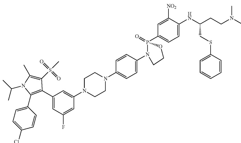
(R)-3-(4-(3-(2-(4-chlorophenyl)-1-isopropyl-5-methyl-4-(methylsulfonyl)-1H-pyrrol-3-yl)-5-fluorophenyl)piperazin-1-yl)phenyl-2-(4-((R)-4-(dimethylamino)-1-(phenylthio)butan-2-yl)amino)-3-nitrophenyl-1,3,2-oxazaphospholidine 2-oxide
