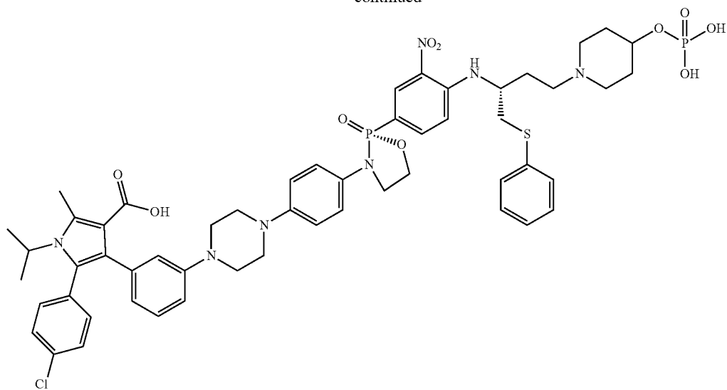
5-(4-chlorophenyl)-1-isopropyl-2-methyl-4-(3-(4-(4-((R)-2-(3-nitro-4-((R)-1-(phenylthio)-4-(4-(phosphonoxy)piperidin-1-yl)butan-2-yl)amino)phenyl)-2-oxido-1,3,2-oxazaphospholidin-3-yl)phenyl)piperazin-1-yl)phenyl)-1H-pyrrole-3-carboxylic acid
