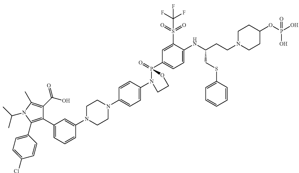
5-(4-chlorophenyl)-1-isopropyl-2-methyl-4-(3-(4-(4-((S)-2-oxido-2-(4-((R)-1-(phenylthio)-4-(4-(phosphonooxy)piperidin-1-yl)butan-2-yl)amino)-3-((trifluoromethyl)sulfonyl)phenyl)-1,3,2-oxazaphospholidin-3-yl)phenyl)piperazin-1-yl)phenyl)-1H-pyrrole-3-carboxylic acid,
