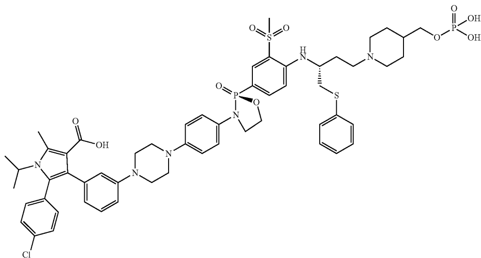
5-(4-chlorophenyl)-1-isopropyl-2-methyl-4-(3-(4-(4-((S)-2-(3-(methylsulfonyl)-4-((R)-1-(phenylthio)-4-(4-(phosphonoxy)piperidin-1-yl)butan-2-yl)amino)phenyl)-2-oxido-1,3,2-oxazaphospholidin-3-yl)phenyl)piperazin-1-yl)phenyl)-1H-pyrrole-3-carboxylic acid
