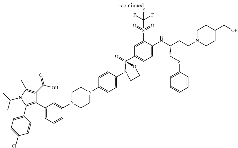
5-(4-chlorophenyl)-4-(3-(4-((S)-2-(4-(((R)-4-(4-(hydroxymethyl)piperidin-1-yl)-1-(phenylthio)butan-2-yl)amino)-3-((trifluoromethyl)sulfonyl)phenyl)-2-oxido-1,3,2-oxazaphospholidin-3-yl)phenyl)piperazin-1-yl)phenyl)-1-isopropyl-2-methyl-1H-pyrrole-3-carboxylic acid,
