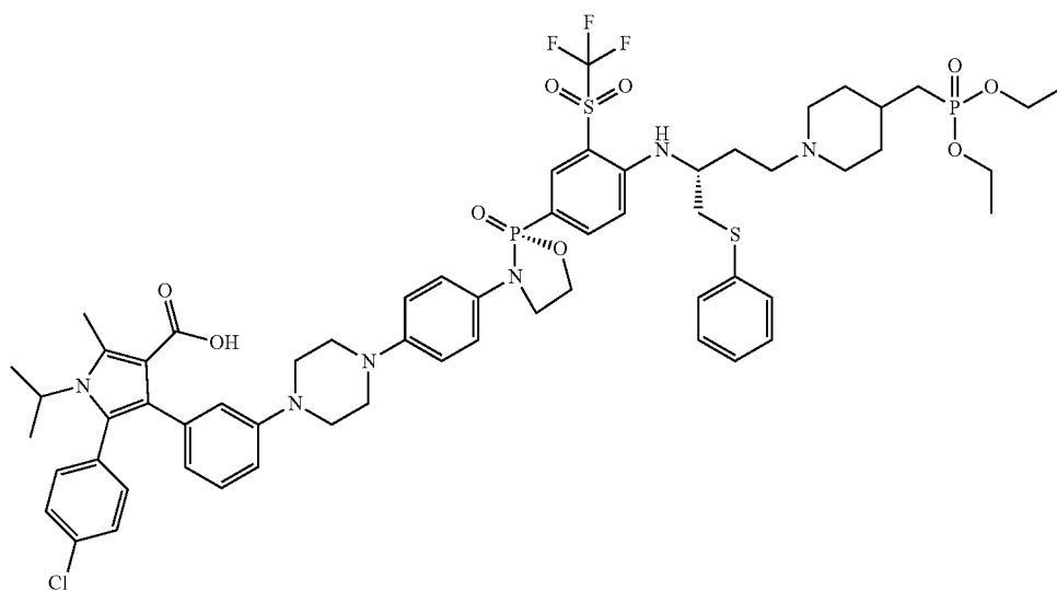
5-(4-chlorophenyl)-4-(3-(4-(4-((R)-2-(4-((R)-4-(4-((diethoxyphosphoryl)methyl)piperidin-1-yl)-1-(phenylthio)butan-2-yl)amino)-3-((trifluoromethyl)sulfonyl)phenyl)-2-oxido-1,3,2-oxazaphospholidin-3-yl)phenyl)piperazin-1-yl)phenyl)-1-isopropyl-2-methyl-1H-pyrrole-3-carboxylic acid
