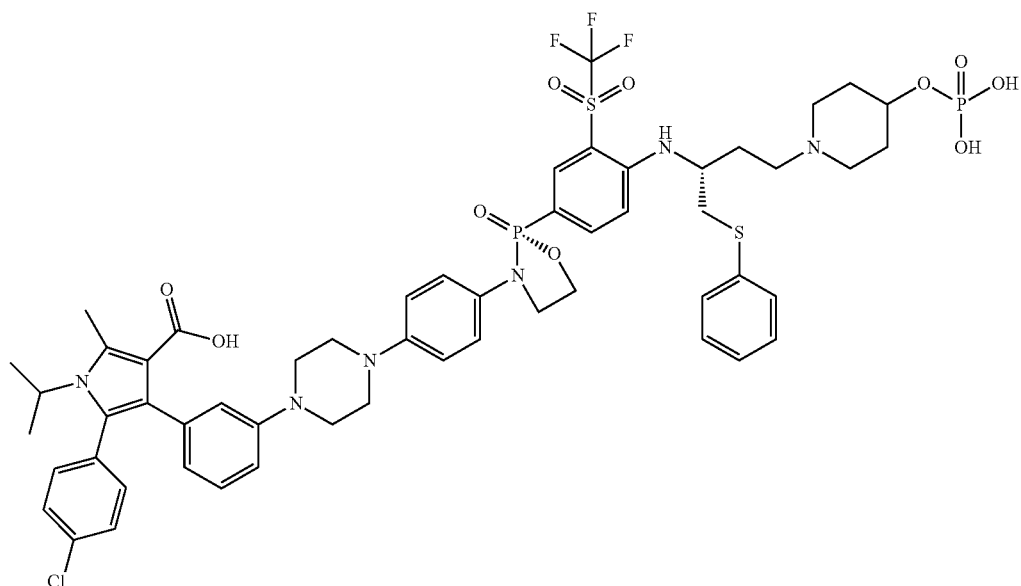
5-(4-chlorophenyl)-1-isopropyl-2-methyl-4-(3-(4-(4-((R)-2-oxido-2-(4-((R)-1-(phenylthio)-4-(4-(phosphonooxy)piperidin-1-yl)butan-2-yl)amino)-3-((trifluoromethyl)sulfonyl)phenyl)-1,3,2-oxazaphospholidin-3-yl)phenyl)piperazin-1-yl)phenyl)-1H-pyrrole-3-carboxylic acid,
