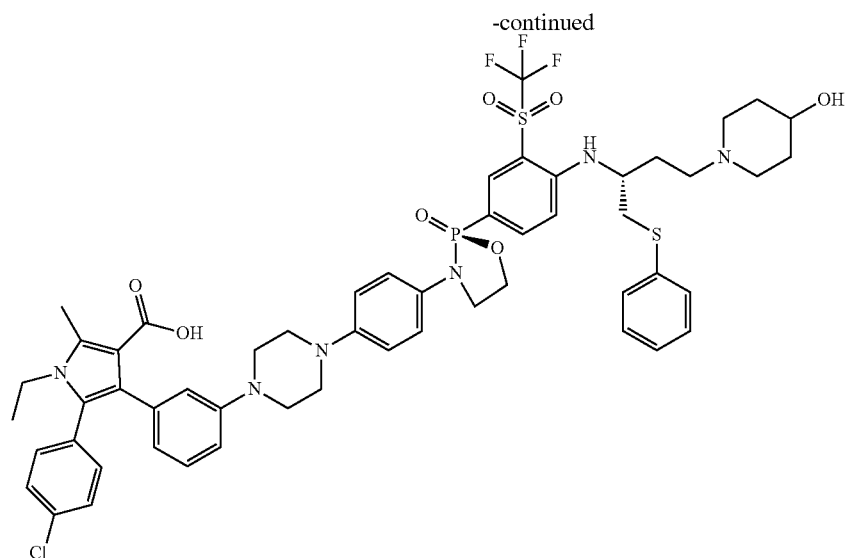
5-(4-chlorophenyl)-1-ethyl-4-(3-(4-(4-((S)-2-(4-(((R)-4-(4-hydroxypiperidin-1-yl)-1-(phenylthio)butan-2-yl)amino)-3-(trifluoromethyl)sulfonyl)phenyl)-2-oxido-1,3,2-oxazaphospholidin-3-yl)phenyl)piperazin-1-yl)phenyl)-2-methyl-1H-pyrrole-3-carboxylic acid
