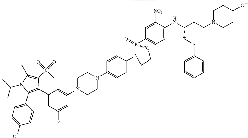
(R)-3-(4-(4-(3-(2-(4-chlorophenyl)-1-isopropyl-5-methyl-4-(methylsulfonyl)-1H-pyrrol-3-yl)-5-fluorophenyl)piperazin-1-yl)phenyl)-2-(4-(((R)-4-(4-(hydroxymethyl)piperidin-1-yl)-1-(phenylthio)butan-2-yl)amino)-3-nitrophenyl)-1,3,2-oxazaphospholidine 2-oxide
