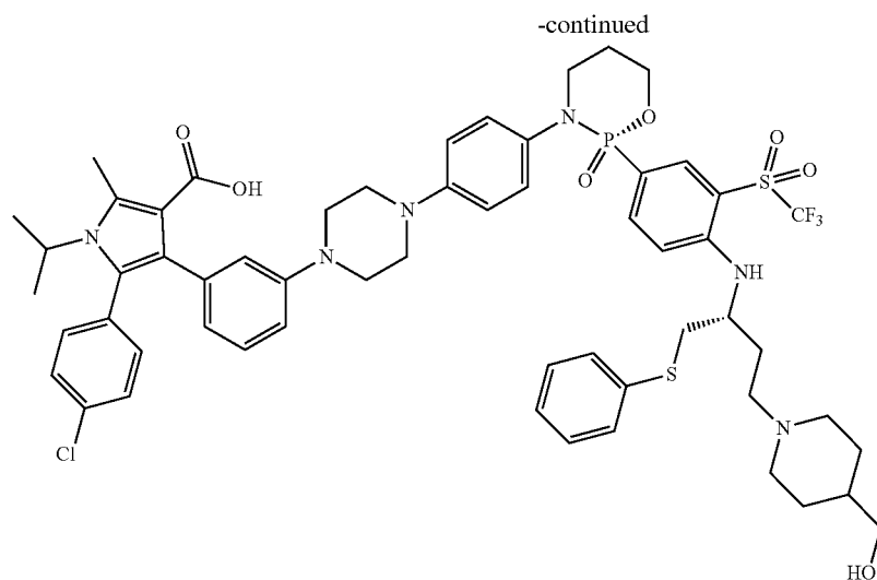
5-(4-chlorophenyl)-4-(3-(4-(4-((S)-2-(4-((R)-4-(4-(hydroxymethyl)piperidin-1-yl)-1-(phenylthio)butan-2-yl)amino)-3-(trifluoromethylsulfonyl)phenyl)-2-oxido-1,3,2-oxazaphosphinan-3-yl)phenyl)piperazin-1-yl)phenyl)-1-isopropyl-2-methyl-1H-pyrrole-3-carboxylic acid
