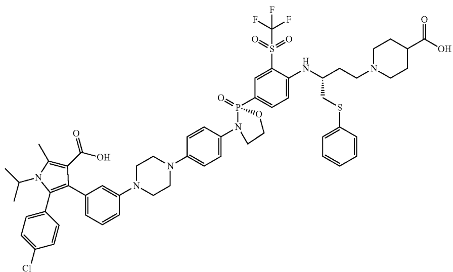
1-((R)-3-((4-((R)-3-(4-(4-(3-(4-carboxy-2-(4-chlorophenyl)-1-isopropyl-5-methyl-1H-pyrrol-3-yl)phenyl)piperazin-1-yl)phenyl)-2-oxido-1,3,2-oxazaphospholidin-2-yl)-2-((trifluoromethyl)sulfonyl)phenyl)amino)-4-(phenylthio)butyl)piperidine-4-carboxylic acid
