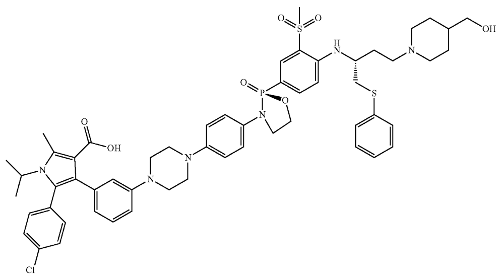
5-(4-chlorophenyl)-4-(3-(4-(4-((S)-2-(4-((R)-4-(4-(hydroxymethyl)piperidin-1-yl)-1-(phenylthio)butan-2-yl)amino)-3-(methylsulfonyl)phenyl)-2-oxido-1,3,2-oxazaphospholidin-3-yl)phenyl)piperazin-1-yl)phenyl)-1-isopropyl-2-methyl-1H-pyrrole-3-carboxylic acid
