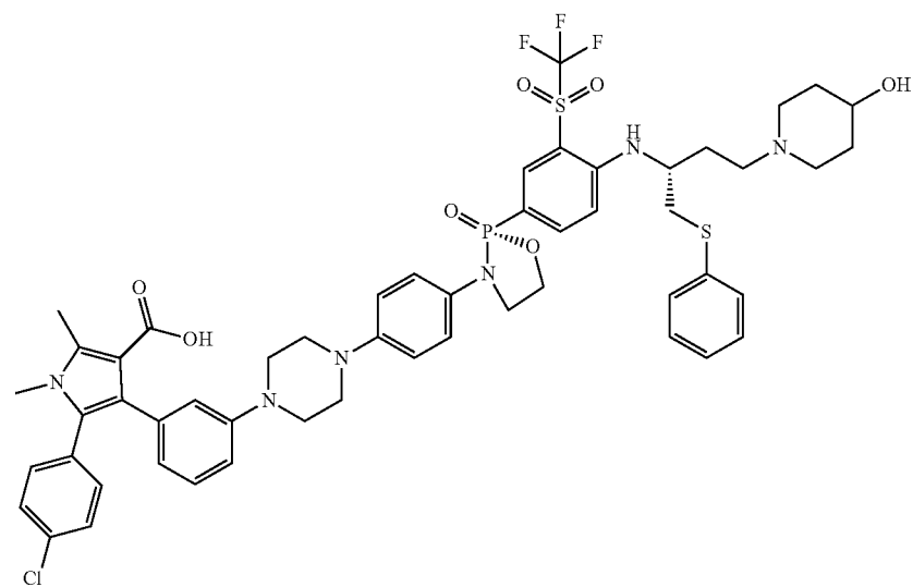
5-(4-chlorophenyl)-4-(3-(4-(4-((R)-2-(4-(((R)-4-(4-hydroxypiperidin-1-yl)-1-(phenylthio)butan-2-yl)amino)-3-(trifluoromethyl)sulfonyl)phenyl)-2-oxido-1,3,2-oxazaphospholidin-3-yl)phenyl)piperazin-1-yl)phenyl)-1,2-dimethyl-1H-pyrrole-3-carboxylic acid
