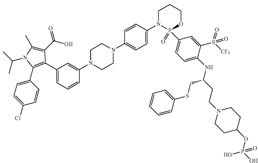
5-(4-chlorophenyl)-1-isopropyl-2-methyl-4-(3-(4-(4-((R)-2-oxido-2-(4-((R)-1-(phenylthio)-4-(4-(phosphonoxy)piperidin-1-yl)butan-2-yl)amino)-3-(trifluoromethyl)sulfonyl)phenyl)-1,3,2-oxazaphosphinan-3-yl)phenyl)piperazin-1-yl)phenyl)-1H-pyrrole-3-carboxylic acid
