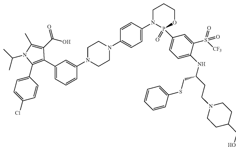
5-(4-chlorophenyl)-4-(3-(4-(4-((R)-2-(4-((R)-4-(4-(hydroxymethyl)piperidin-1-yl)-1-(phenylthio)butan-2-yl)amino)-3-(trifluoromethylsulfonyl)phenyl)-2-oxido-1,3,2-oxazaphosphinan-3-yl)phenyl)piperazin-1-yl)phenyl)-1-isopropyl-2-methyl-1H-pyrrole-3-carboxylic acid
