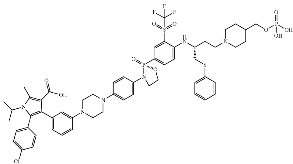
5-(4-chlorophenyl)-1-isopropyl-2-methyl-4-(3-(4-(4-((R)-2-oxido-2-(4-((R)-1-(phenylthio)-4-(4-((phosphonoxy)methyl)piperidin-1-yl)butan-2-yl)amino)-3-((trifluoromethyl)sulfonyl)phenyl)-1,3,2-oxazaphospholidin-3-yl)phenyl)piperazin-1-yl)phenyl)-1H-pyrrole-3-carboxylic acid
