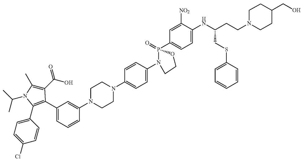
5-(4-chlorophenyl)-4-(3-(4-(4-((R)-2-(4-(((R)-4-(4-(hydroxymethyl)piperidin-1-yl)-1-(phenylthio)butan-2-yl)amino)-3-nitrophenyl)-2-oxido-1,3,2-oxazaphospholidin-3-yl)phenyl)piperazin-1-yl)phenyl)-1-isopropyl-2-methyl-1H-pyrrole-3-carboxylic acid
