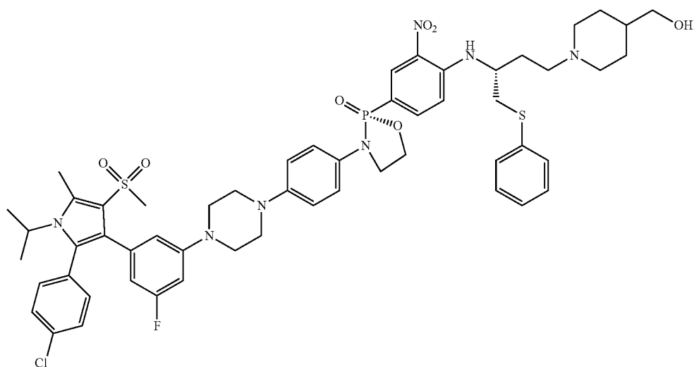
(R)-3-(4-(4-(3-(2-(4-chlorophenyl)-1-isopropyl-5-methyl-4-(methylsulfonyl)-1H-pyrrol-3-yl)-5-fluorophenyl)piperazin-1-yl)phenyl)-2-4-(((R)-4-(4-(hydroxymethyl)piperidin-1-yl)-1-(phenylthio)butan-2-yl)amino)-3-nitrophenyl)-1,3,2-oxazaphospholidine 2-oxide
