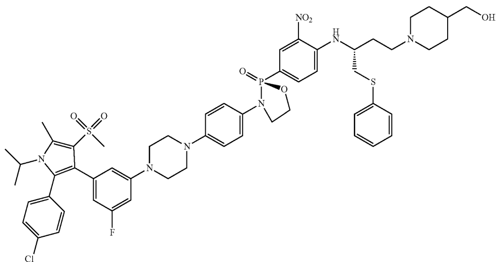
(S)-3-(4-(4-(3-(2-(4-chlorophenyl)-1-isopropyl-5-methyl-4-(methylsulfonyl)-1H-pyrrol-3-yl)-5-fluorophenyl)piperazin-1-yl)phenyl)-2-4-(((S)-4-(4-(hydroxymethyl)piperidin-1-yl)-1-(phenylthio)butan-2-yl)amino)-3-nitrophenyl)-1,3,2-oxazaphospholidine 2-oxide
