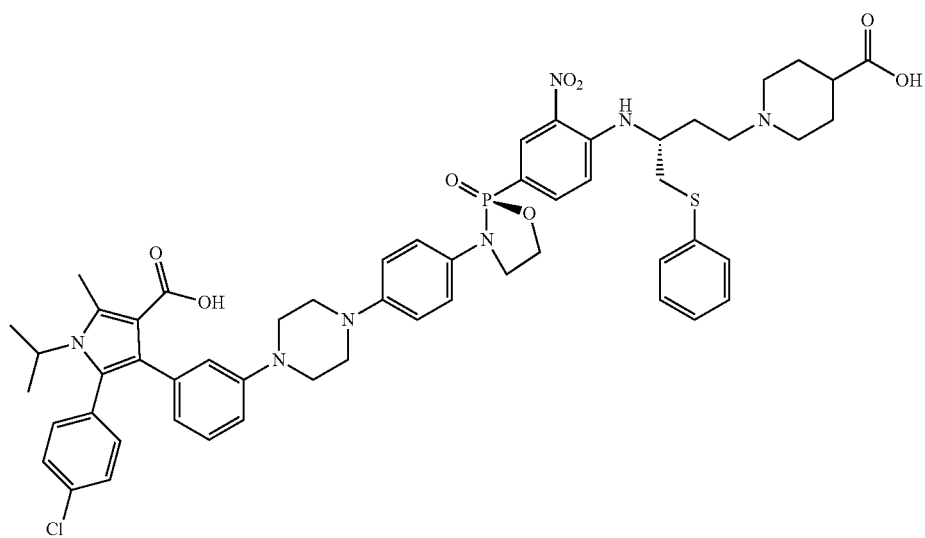
1-((S)-3-((4-((R)-3-(4-(4-(3-(4-carboxy-2-(4-chlorophenyl)-1-isopropyl-5-methyl-1H-pyrrol-3-yl)phenyl)piperazin-1-yl)phenyl)-2-oxido-1,3,2-oxazaphospholidin-2-yl)-1-nitrophenyl)amino)-4-(phenylthio)butyl)piperidine-4-carboxylic acid
