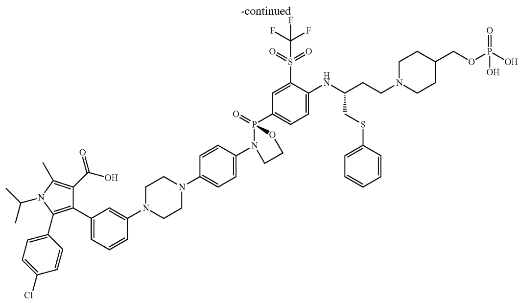
5-(4-chlorophenyl)-1-isopropyl-2-methyl-4-(3-(4-(4-((S)-2-oxido-2-(4-((R)-1-(phenylthio)-4-(4-(phosphonoxy)methyl)piperidin-1-yl)butan-2-yl)amino-3-((trifluoromethyl)sulfonyl)phenyl)-1,3,2-oxazaphospholidin-3-yl)phenyl)piperazin-1-yl)phenyl)-1H-pyrrole-3-carboxylic acid,
