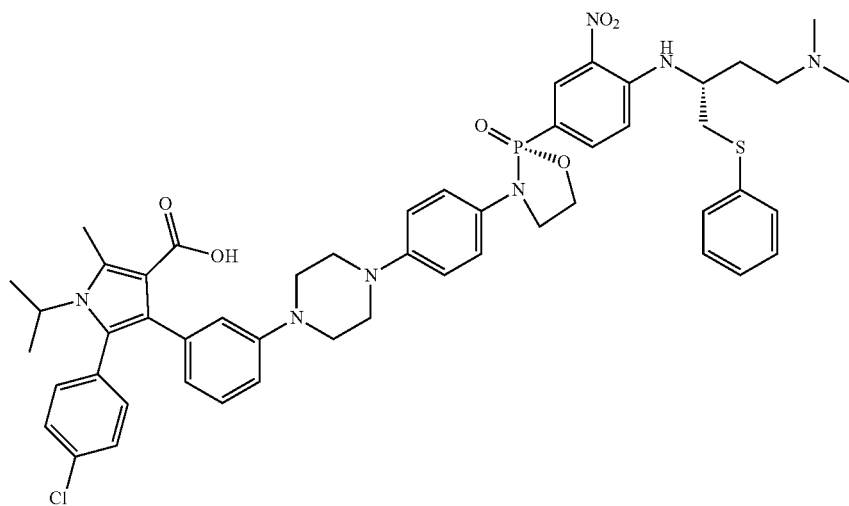
5-(4-chlorophenyl)-4-(3-(4-(4-(((R)-2-(4-(((R)-4-(dimethylamino)-1-(phenylthio)butan-2-yl)amino)-3-nitrophenyl)-2-oxido-1,3,2-oxazaphospholidin-3-yl)phenyl)piperazin-1-yl)phenyl)-1-isopropyl-2-methyl-1H-pyrrole-3-carboxylic acid
