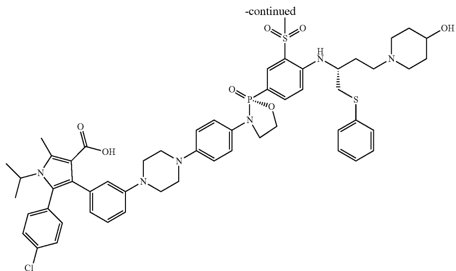
5-(4-chlorophenyl)-4-(3-(4-(4-((R)-2-(4-((R)-4-(4-(hydroxypiperidin-1-yl)-1-(phenylthio)butan-2-yl)amino)-3-(methylsulfonyl)phenyl)-2-oxido-1,3,2-oxazaphospholidin-3-yl)phenyl)piperazin-1-yl)phenyl)-1-isopropyl-2-methyl-1H-pyrrole-3-carboxylic acid
