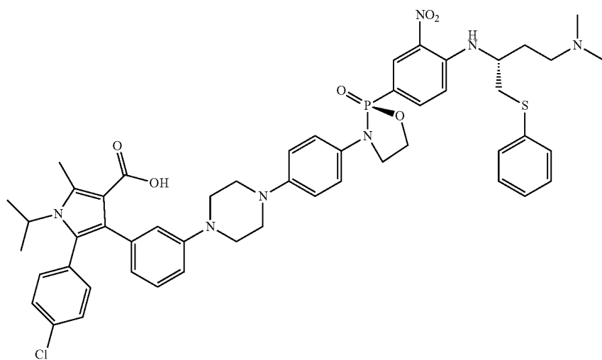
5-(4-chlorophenyl)-4-(3-(4-(4-((S)-2-((S)-2-(4-(((R)-4-(dimethylamino)-1-(phenylthio)butan-2-yl)amino)-3-nitrophenyl)-2-oxido-1,3,2-oxazaphospholidin-3-yl)phenyl)piperazin-1-yl)phenyl)-1-isopropyl-2-methyl-1H-pyrrole-3-carboxylic acid
