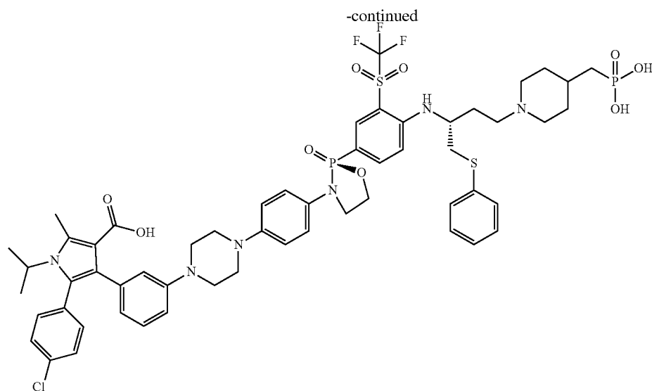
5-(4-chlorophenyl)-1-isopropyl-2-methyl-4-(3-(4-(4-((S)-2-oxido-2-(4-(((R)-1-(phenylthio)-4-(4-(phosphonomethyl)piperidin-1-yl)butan-2-yl)amino)-3-(trifluoromethyl)sulfonyl)phenyl)-1,3,2-oxazaphospholidin-3-yl)phenyl)piperazin-1-yl)phenyl)-1H-pyrrole-3-carboxylic acid
