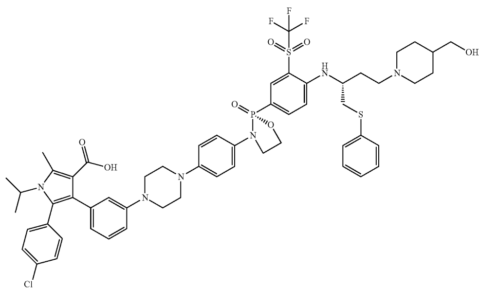
5-(4-chlorophenyl)-4-(3-(4-(4-((R)-2-(4-((R)-4-(4-hydroxymethyl)piperidin-1-yl)-1-(phenylthio)butan-2-yl)amino)-3-((trifluoromethyl)sulfonyl)phenyl)-2-oxido-1,3,2-oxazaphospholidin-3-yl)phenyl)piperazin-1-yl)phenyl)-1-isopropyl-2-methyl-1H-pyrrole-3-carboxylic acid,
