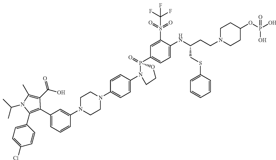
5-(4-chlorophenyl)-1-isopropyl-2-methyl-4-(3-(4-(4-((R)-2-oxido-2-(4-((R)-1-(phenylthio)-4-(4-(phosphonoxy)piperidin-1-yl)butan-2-yl)amino)-3-((trifluoromethyl)sulfonyl)phenyl)-1,3,2-oxazaphospholidin-3-yl)phenyl)piperazin-1-yl)phenyl)-1H-pyrrole-3-carboxylic acid
