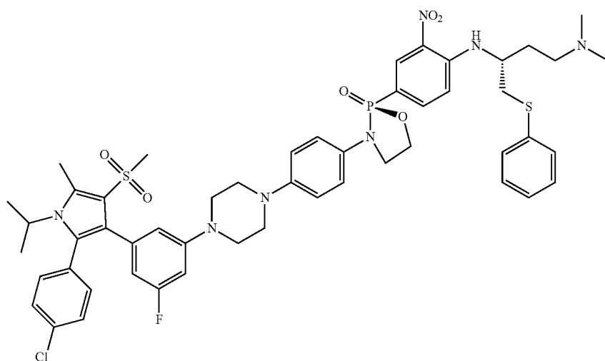
(S)-3-(4-(3-(2-(4-chlorophenyl)-1-isopropyl-5-methyl-4-(methylsulfonyl)-1H-pyrrol-3-yl)-5-fluorophenyl)piperazin-1-yl)phenyl-2-(4-((R)-4-(dimethylamino)-1-(phenylthio)butan-2-yl)amino)-3-nitrophenyl-1,3,2-oxazaphospholidine 2-oxide
