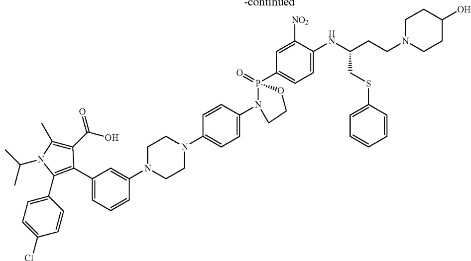
5-(4-chlorophenyl)-4-(3-(4-(4-((R)-2-(4-(((R)-2-(4-(((R)-4-(4-hydroxypiperidin-1-yl)-1-(phenylthio)butan-2-yl)amino)-3-nitrophenyl)-2-oxido-1,3,2-oxazaphospholidin-3-yl)phenyl)piperazin-1-yl)phenyl)-1-isopropyl-2-methyl-1H-pyrrole-3-carboxylic acid
