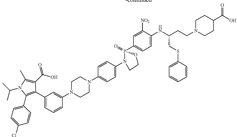
1-((R)-3-((4-((R)-3-(4-(4-(3-(4-carboxy-2-(4-chlorophenyl)-1-isopropyl-5-methyl-1H-pyrrol-3-yl)phenyl)piperazin-1-yl)phenyl)-2-oxido-1,3,2-oxazaphospholidin-2-yl)-1-nitrophenyl)amino)-4-(phenylthio)butyl)piperidine-4-carboxylic acid
