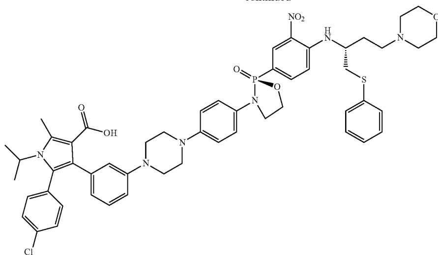
5-(4-chlorophenyl)-1-isopropyl-2-methyl-4-(3-(4-(4-((S)-2-(4-((R)-4-morpholino-1-(phenylthio)butan-2-yl)amino)-3-nitrophenyl)-2-oxido-1,3,2-oxazaphospholidin-3-yl)phenyl)piperazin-1-yl)phenyl)-1H-pyrrole-3-carboxylic acid
