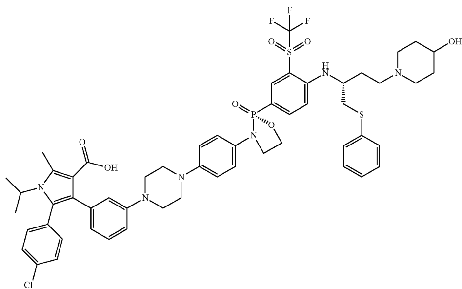
5-(4-chlorophenyl)-4-(3-(4-(4-((R)-2-(4-((R)-4-(4-hydroxypiperidin-1-yl)-1-(phenylthio)butan-2-yl)amino)-3-((trifluoromethyl)sulfonyl)phenyl)-2-oxido-1,3,2-oxazaphospholidin-3-yl)phenyl)piperazin-1-yl)phenyl)-1-isopropyl-2-methyl-1H-pyrrole-3-carboxylic acid,
