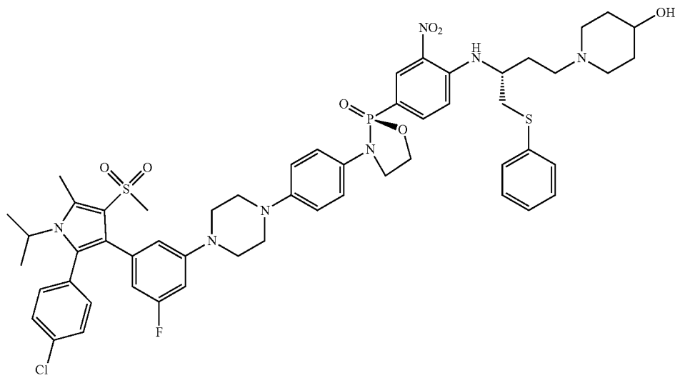
(S)-3-(4-(4-(3-(2-(4-chlorophenyl)-1-isopropyl-5-methyl-4-(methylsulfonyl)-1H-pyrrol-3-yl)-5-fluorophenyl)piperazin-1-yl)phenyl)-2-(4-(((R)-4-(4-(hydroxymethyl)piperidin-1-yl)-1-(phenylthio)butan-2-yl)amino)-3-nitrophenyl)-1,3,2-oxazaphospholidine 2-oxide
