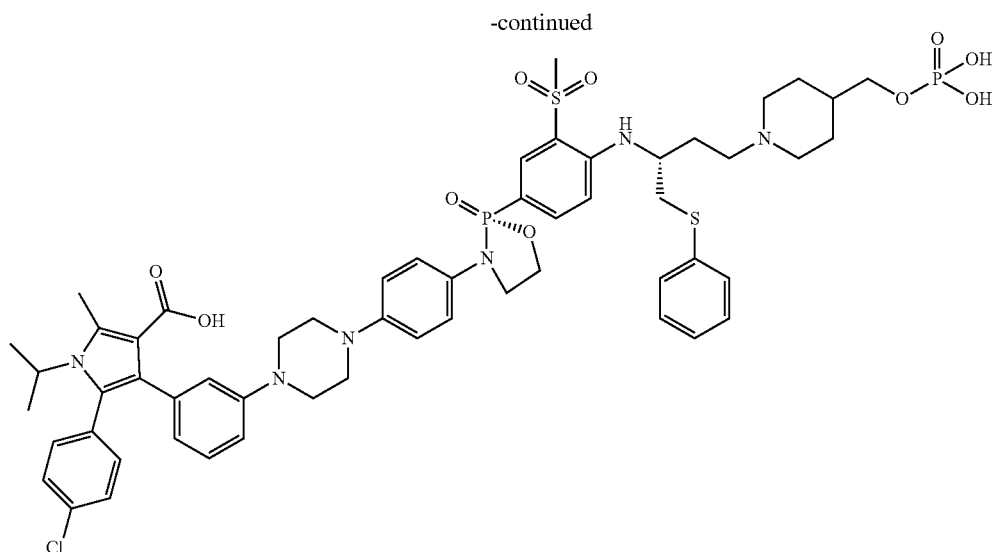
5-(4-chlorophenyl)-1-isopropyl-2-methyl-4-(3-(4-(4-((R)-2-(3-(methylsulfonyl)-4-(((R)-1-(phenylthio)-4-(4-((phosphonoxy)piperidin-1-yl)butan-2-yl)amino)phenyl)-2-oxido-1,3,2-oxazaphospholidin-3-yl)phenyl)piperazin-1-yl)phenyl)-1H-pyrrole-3-carboxylic acid
