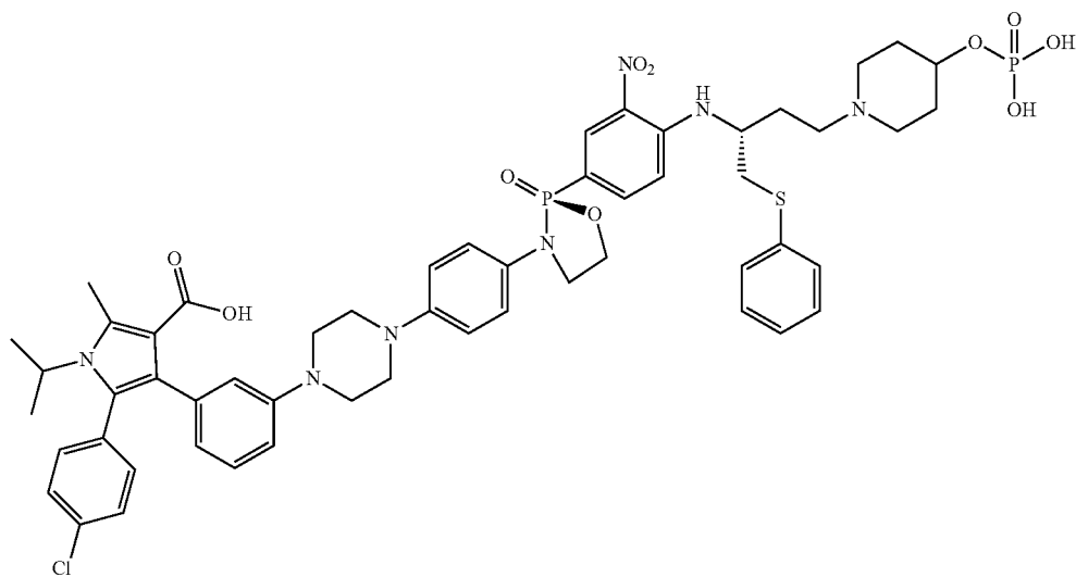
5-(4-chlorophenyl)-1-isopropyl-2-methyl-4-(3-(4-(4-((S)-2-(3-nitro-4-(((R)-1-(phenylthio)-4-(4-(phosphonoxy)piperidin-1-yl)butan-2-yl)amino)phenyl)-2-oxido-1,3,2-oxazaphospholidin-3-yl)phenyl)piperazin-1-yl)phenyl)-1H-pyrrole-3-carboxylic acid
