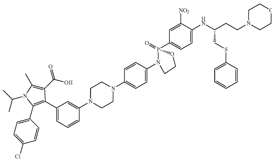
5-(4-chlorophenyl)-1-isopropyl-2-methyl-4-(3-(4-(4-((R)-2-(4-((R)-4-morpholino-1-(phenylthio)butan-2-yl)amino)-3-nitrophenyl)-2-oxido-1,3,2-oxazaphospholidin-3-yl)phenyl)piperazin-1-yl)phenyl)-1H-pyrrole-3-carboxylic acid
