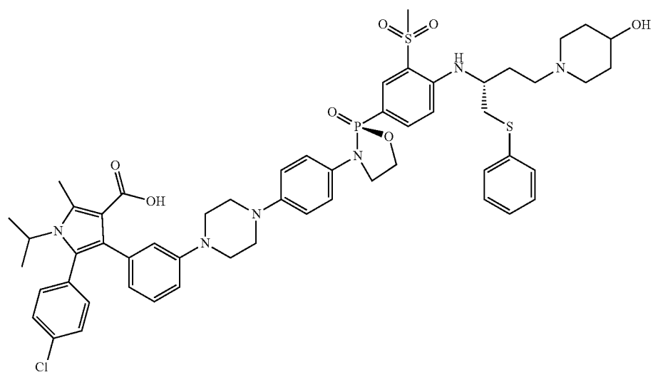
5-(4-chlorophenyl)-4-(3-(4-(4-((S)-2-(4-((R)-4-(4-(hydroxypiperidin-1-yl)-1-(phenylthio)butan-2-yl)amino)-3-(methylsulfonyl)phenyl)-2-oxido-1,3,2-oxazaphospholidin-3-yl)phenyl)piperazin-1-yl)phenyl)-1-isopropyl-2-methyl-1H-pyrrole-3-carboxylic acid
