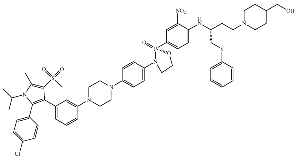
(R)-3-(4-(4-(3-(2-(4-chlorophenyl)-1-isopropyl-5-methyl-4-(methylsulfonyl)-1H-pyrrol-3-yl)phenyl)piperazin-1-yl)phenyl)-2-(4-(((R)-4-(4-(hydroxymethyl)pyridin-1-yl)-1-(phenylthio)butan-2-yl)amino)-3-nitrophenyl)-1,3,2-oxazaphospholidine 2-oxide
