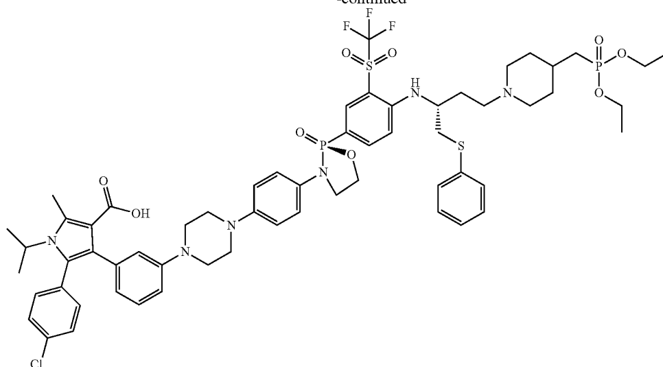
5-(4-chlorophenyl)-4-(3-(4-(4-((S)-2-(4-((R)-4-(4-((diethoxyphosphoryl)methyl)piperidin-1-yl)-1-(phenylthio)butan-2-yl)amino)-3-((trifluoromethyl)sulfonyl)phenyl)-2-oxido-1,3,2-oxazaphospholidin-3-yl)phenyl)piperazin-1-yl)phenyl)-1-isopropyl-2-methyl-1H-pyrrole-3-carboxylic acid
