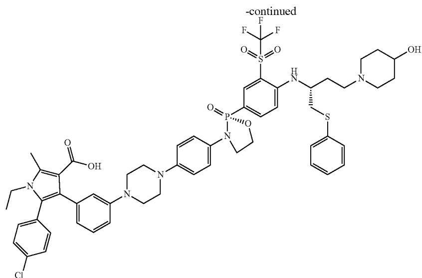
5-(4-chlorophenyl)-1-ethyl-4-(3-(4-(4-((R)-2-(4-((R)-4-(4-hydroxypiperidin-1-yl)-1-(phenylthio)butan-2-yl)amino)-3-(trifluoromethyl)sulfonyl)phenyl)-2-oxido-1,3,2-oxazaphospholidin-3-yl)phenyl)piperazin-1-yl)phenyl)-2-methyl-1H-pyrrole-3-carboxylic acid
