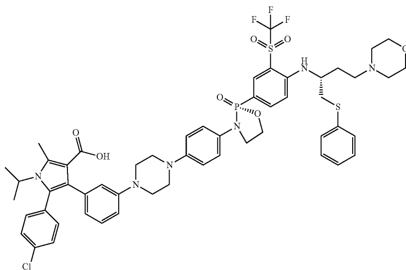
5-(4-chlorophenyl)-1-isopropyl-2-methyl-4-(3-(4-(4-((R)-2-(4-((R)-4-morpholino-1-(phenylthio)butan-2-yl)amino)-3-((trifluoromethyl)sulfonyl)phenyl)-2-oxido-1,3,2-oxazaphospholidin-3-yl)phenyl)piperazin-1-yl)phenyl)-1H-pyrrole-3-carboxylic acid
