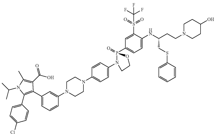
5-(4-chlorophenyl)-4-(3-(4-(4-((S)-2-(4-((R)-4-((R)-4-(4-hydroxypiperidin-1-yl)-1-(phenylthio)butan-2-yl)amino)-3-((trifluoromethyl)sulfonyl)phenyl)-2-oxido-1,3,2-oxazaphospholidin-3-yl)phenyl)piperazin-1-yl)phenyl)-1-isopropyl-2-methyl-1H-pyrrole-3-carboxylic acid
