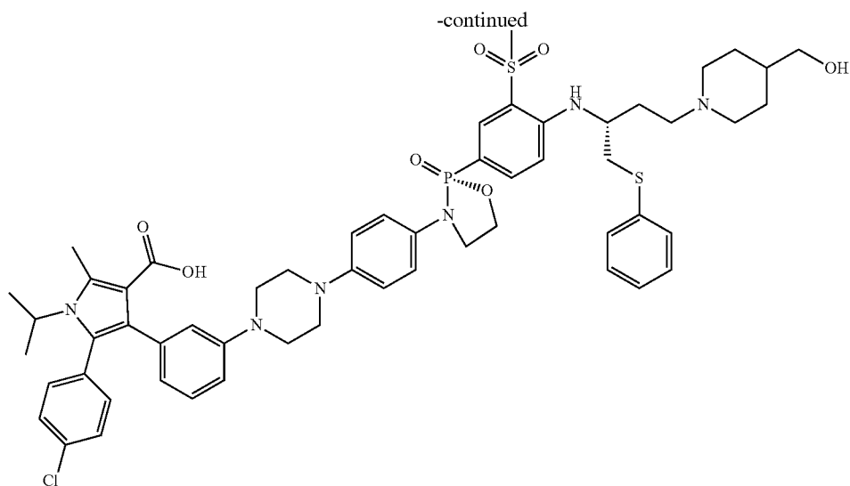
5-(4-chlorophenyl)-4-(3-(4-(4-((R)-2-(4-((R)-4-(4-(hydroxymethyl)piperidin-1-yl)-1-(phenylthio)butan-2-yl)amino)-3-(methylsulfonyl)phenyl)-2-oxido-1,3,2-oxazaphospholidin-3-yl)phenyl)piperazin-1-yl)phenyl)-1-isopropyl-2-methyl-1H-pyrrole-3-carboxylic acid
