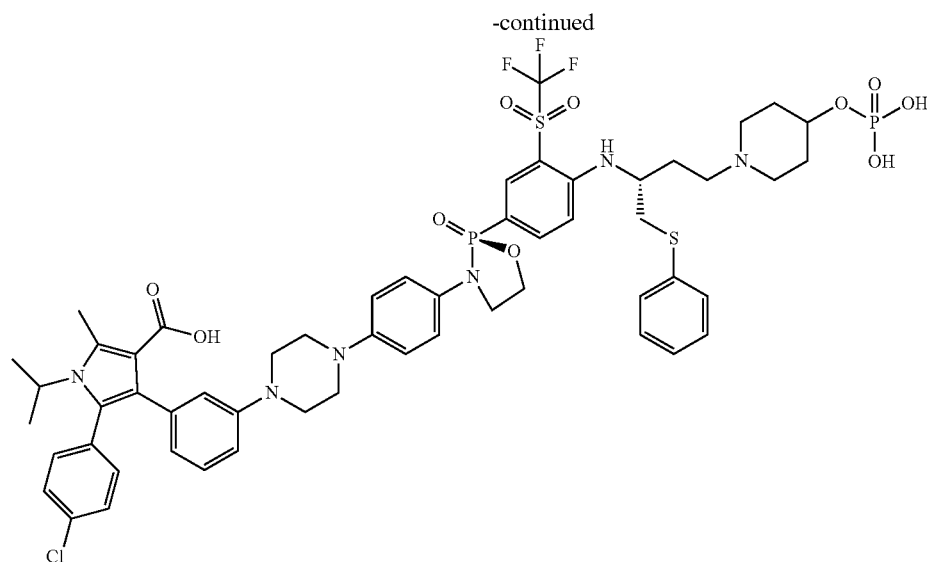
5-(4-chlorophenyl)-1-isopropyl-2-methyl-4-(3-(4-(4-((S)-2-oxido-2-(4-((R)-1-(phenylthio)-4-(4-(phosphonoxy)piperidin-1-yl)butan-2-yl)amino)-3-((trifluoromethyl)sulfonyl)phenyl)-1,3,2-oxazaphospholidin-3-yl)phenyl)piperazin-1-yl)phenyl)-1H-pyrrole-3-carboxylic acid
