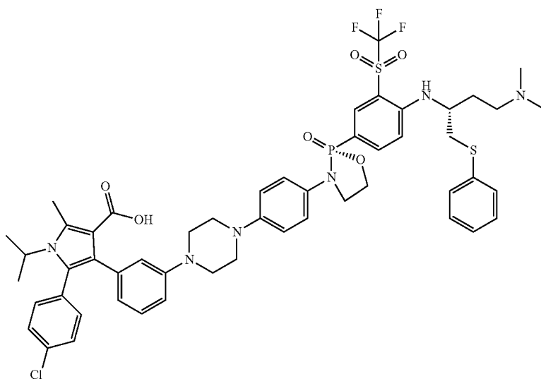
5-(4-chlorophenyl)-4-(3-(4-(4-((R)-2-(4-((R)-4-dimethylamino-1-(phenylthio)butan-2-yl)amino)-3-((trifluoromethyl)sulfonyl)phenyl)-2-oxido-1,3,2-oxazaphospholidin-3-yl)phenyl)piperazin-1-yl)phenyl)-1-isopropyl-2-methyl-1H-pyrrole-3-carboxylic acid
