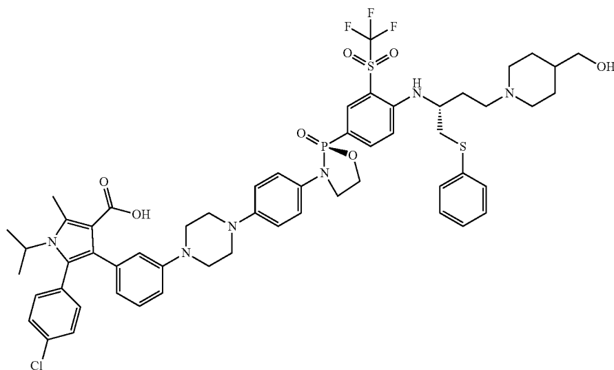
5-(4-chlorophenyl)-4-(3-(4-(4-((S)-2-(4-((R)-4-((R)-4-(4-hydroxypiperidin-1-yl)-1-(phenylthio)butan-2-yl)amino)-3-(trifluoromethyl)sulfonyl)phenyl)-2-oxido-1,3,2-oxazaphospholidin-3-yl)phenyl)piperazin-1-yl)phenyl)-1-isopropyl-2-methyl-1H-pyrrole-3-carboxylic acid
