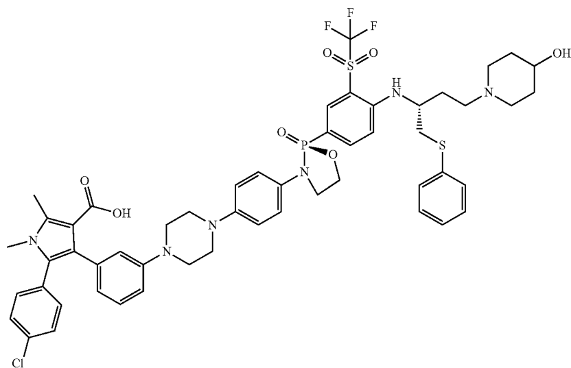
5-(4-chlorophenyl)-1-ethyl-4-(3-(4-(4-((S)-2-(4-((R)-4-(4-hydroxypiperidin-1-yl)-1-(phenylthio)butan-2-yl)amino)-3-(trifluoromethyl)sulfonyl)phenyl)-2-oxido-1,3,2-oxazaphospholidin-3-yl)phenyl)piperazin-1-yl)phenyl)-2-dimethyl-1H-pyrrole-3-carboxylic acid
