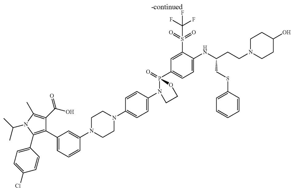
5-(4-chlorophenyl)-4-(3-(4-(4-((S)-2-(4-((R)-4-(4-hydroxypiperidin-1-yl)-1-(phenylthio)butan-2-yl)amino)-3-((trifluoromethyl)sulfonyl)phenyl)-2-oxido-1,3,2-oxazaphospholidin-3-yl)phenyl)piperazin-1-yl)phenyl)-1-isopropyl-2-methyl-1H-pyrrole-3-carboxylic acid,
