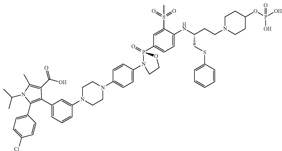
5-(4-chlorophenyl)-1-isopropyl-2-methyl-4-(3-(4-(4-((S)-2-(3-(methylsulfonyl)-4-((R)-1-(phenylthio)-4-(4-(phosphonoxy)piperidin-1-yl)butan-2-yl)amino)phenyl)-2-oxido-1,3,2-oxazaphospholidin-3-yl)phenyl)piperazin-1-yl)phenyl)-1H-pyrrole-3-carboxylic acid
