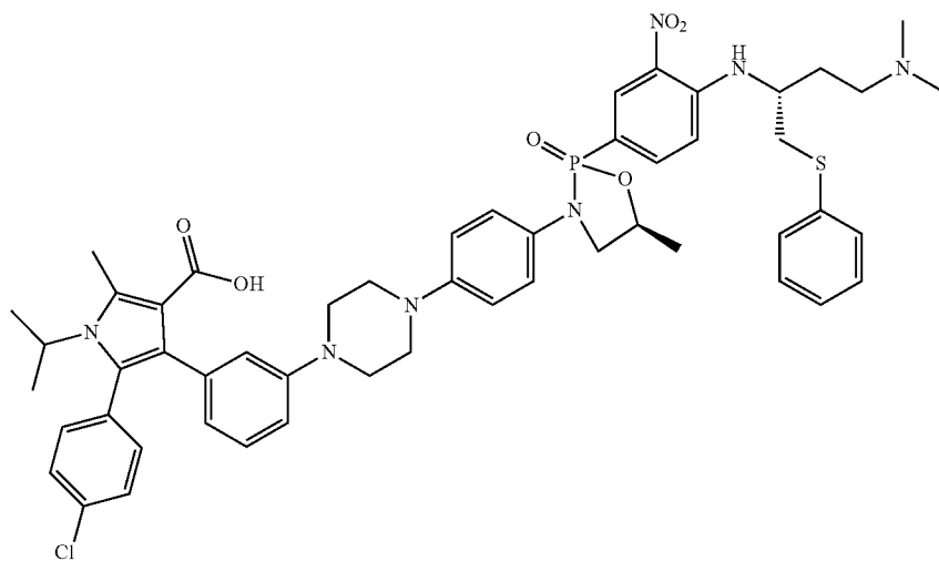
5-(4-chlorophenyl)-4-(3-(4-(4-((5S)-2-(4-((R)-4-dimethylamino)-1-(phenylthio)butan-2-yl)amino-3-nitrophenyl)-5-methyl-2-oxido-1,3,2-oxazaphospholidin-3-yl)phenyl)piperazin-1-yl)phenyl)-1-isopropyl-2-methyl-1H-pyrrole-3-carboxylic acid
