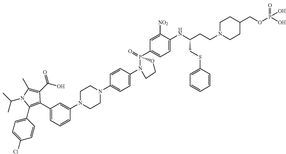
5-(4-chlorophenyl)-1-isopropyl-2-methyl-4-(3-(4-(4-((R)-2-(3-nitro-4-((R)-1-(phenylthio)-4-(4-((phosphonoxy)methyl)piperidin-1-yl)butan-2-yl)amino)phenyl)-2-oxido-1,3,2-oxazaphospholidin-3-yl)phenyl)piperazin-1-yl)phenyl)-1H-pyrrole-3-carboxylic acid
