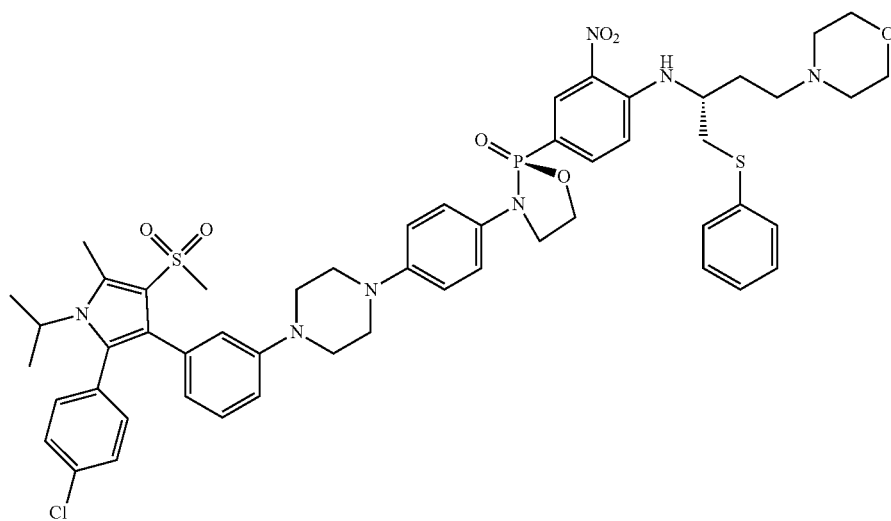
(S)-3-(4-(4-(3-(2-(4-chlorophenyl)-1-isopropyl-5-methyl-4-(methylsulfonyl)-1H-pyrrol-3-yl)phenyl)piperazin-1-yl)phenyl)-2-(4-(((S)-4-morpholino-1-(phenylthio)butan-2-yl)amino)-3-nitrophenyl)-1,3,2-oxazaphospholidine 2-oxide
