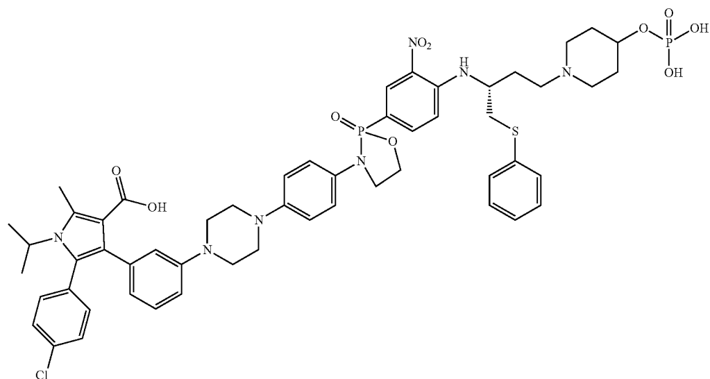
5-(4-chlorophenyl)-1-isopropyl-2-methyl-4-(3-(4-(4-(2-(3-nitro-4-((R)-1-(phenylthio)-4-(4-(phosphonoxy)piperidin-1-yl)butan-2-yl)amino)phenyl)-2-oxido-1,3,2-oxazaphospholidin-3-yl)phenyl)piperazin-1-yl)phenyl)-1H-pyrrole-3-carboxylic acid
