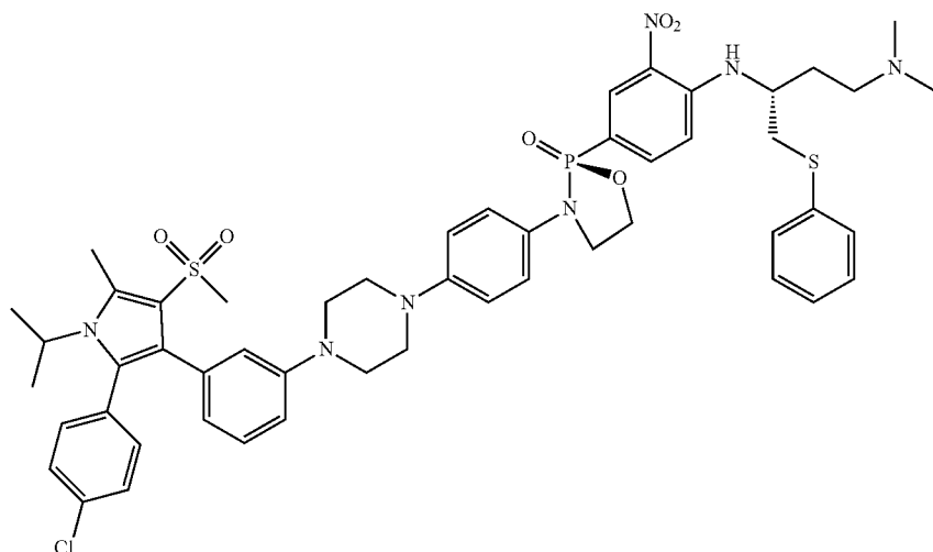
(S)-3-(4-(4-(3-(2-(4-chlorophenyl)-1-isopropyl-5-methyl-4-(methylsulfonyl)-1H-pyrrol-3-yl)phenyl)piperazin-1-yl)phenyl)-2-(4-(((R)-4-(dimethylamino)-1-(phenylthio)butan-2-yl)amino)-3-nitrophenyl)-1,3,2-oxazaphospholidine 2-oxide
