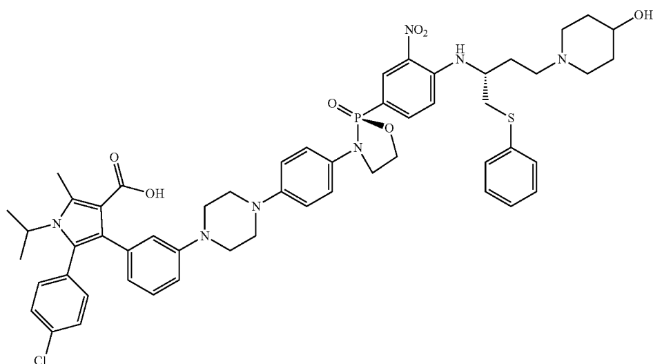
5-(4-chlorophenyl)-4-(3-(4-(4-((S)-2-(4-(((R)-4-(4-hydroxypiperidin-1-yl)-1-(phenylthio)butan-2-yl)amino)-3-nitrophenyl)-2-oxido-1,3,2-oxazaphospholidin-3-yl)phenyl)piperazin-1-yl)phenyl)-1-isopropyl-2-methyl-1H-pyrrole-3-carboxylic acid
