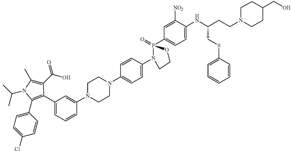
5-(4-chlorophenyl)-4-(3-(4-(4-((S)-2-(4-(((R)-4-(4-hydroxymethyl)piperidin-1-yl)-1-(phenylthio)butan-2-yl)amino)-3-nitrophenyl)-2-oxido-1,3,2-oxazaphospholidin-3-yl)phenyl)piperazin-1-yl)phenyl)-1-isopropyl-2-methyl-1H-pyrrole-3-carboxylic acid
