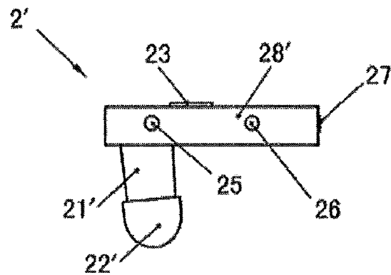
C-C View
