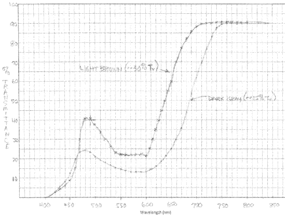
Therapeutic Lens Transmittance Curves
