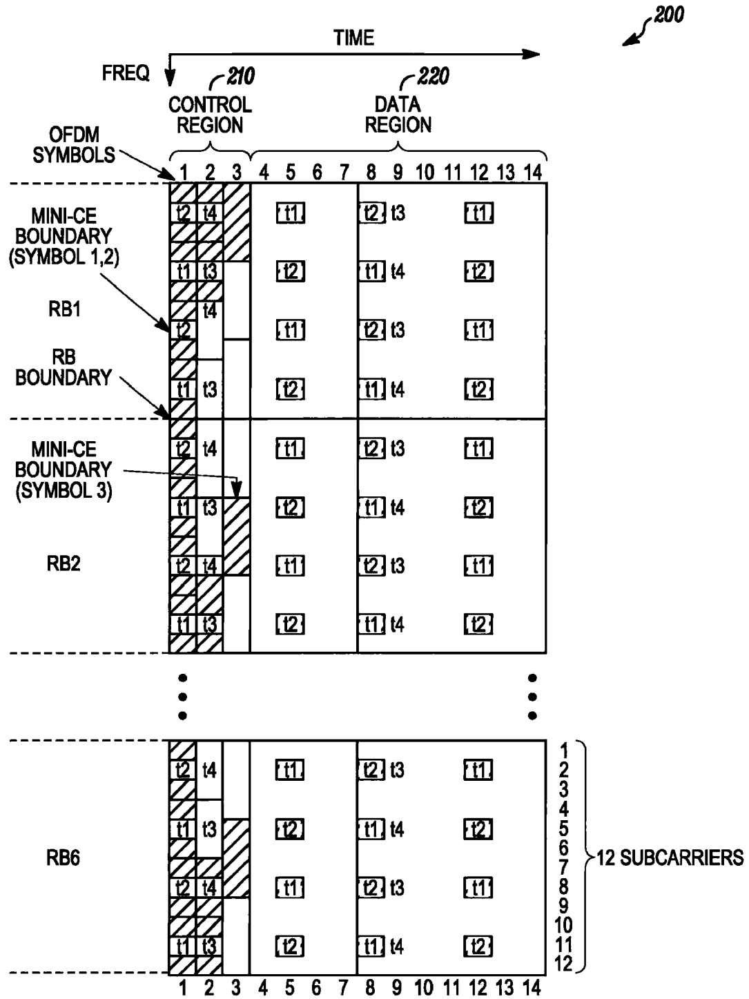
FDD DOWNLINK SUB-FRAME FOR 1.25 MHz CARRIER
