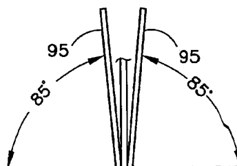
VIEW A-A TILT OF BACK WHEELS
