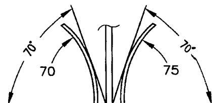
VIEW A-A TILT OF FRONT WHEELS
