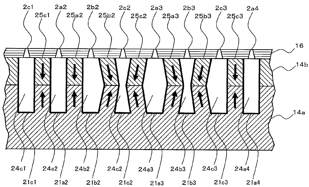
B-B SECTION
