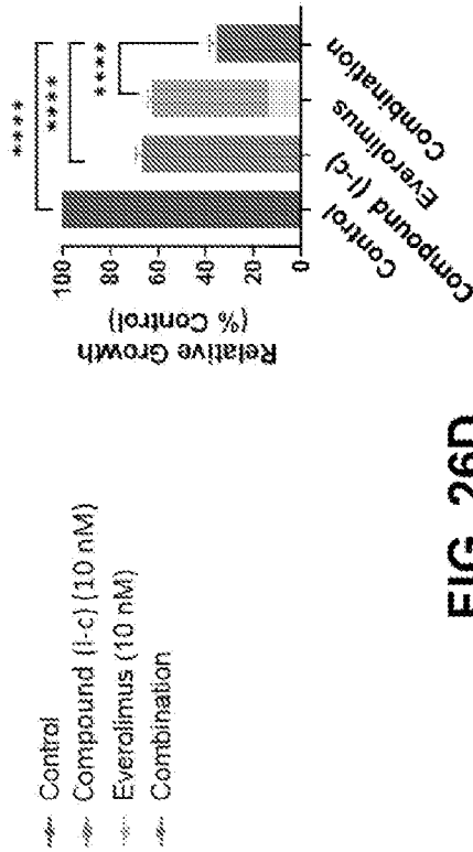
FIG. 26B Relative Cell Growth at 120 Hours
