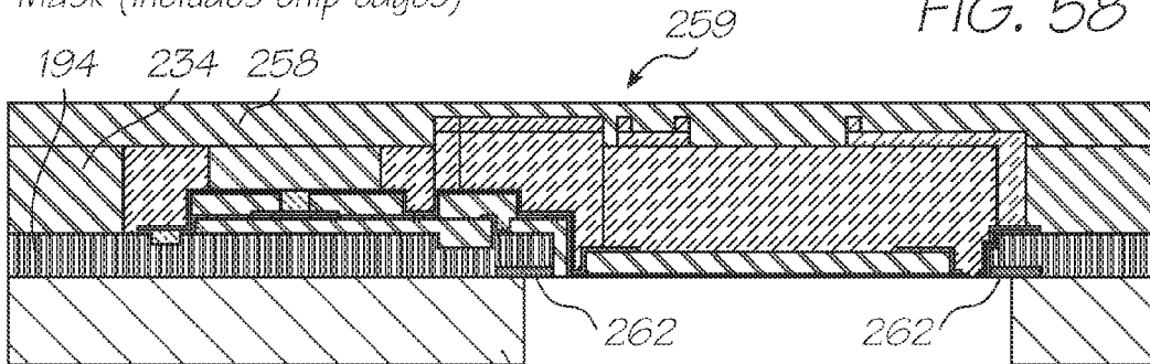
Back-etch using Bosch process
