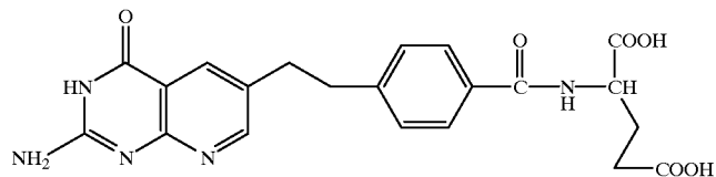
5,10-dideaza tetrahydrofolate
