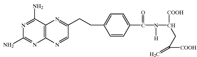
\gamma -methylene-10-deaza aminopterin (MDAM)
