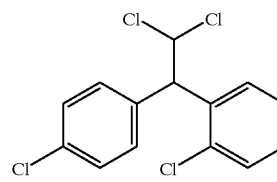
Mitotane
