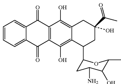
Idarubicin
