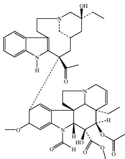
Vincristine
