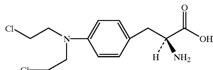
Melphalan
