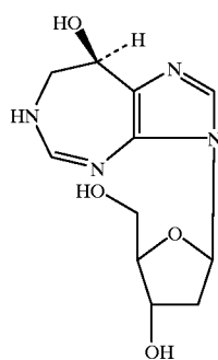
Pentostatin
