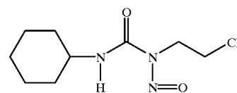
Lomustine (CCNU)
