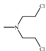
Mechlorethamine
