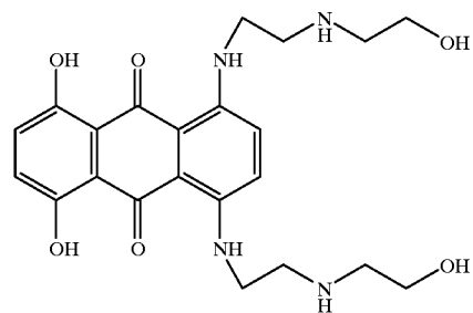
Mitoxantrone
