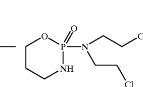
Cyclophosphamide
