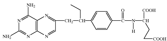
10-ethyl-10-deaza aminopterin (EDAM)
