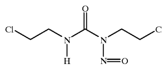
Carmustine (BCNU)
