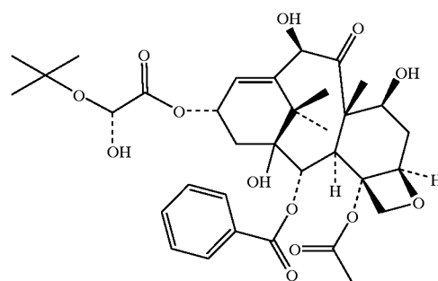
Taxotere
