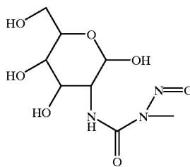
Streptozocin
