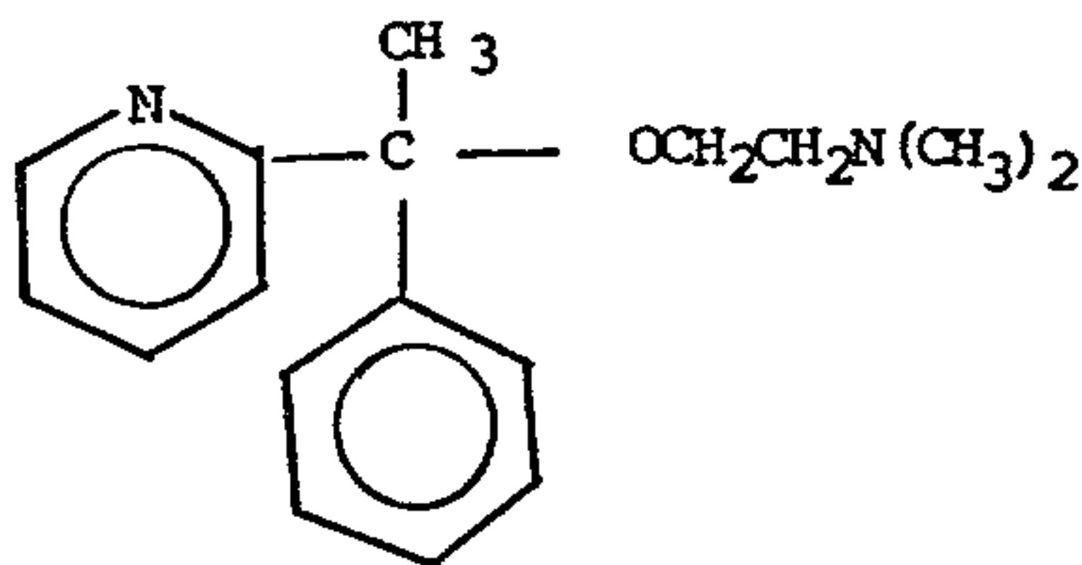
Doxylamine succinate
