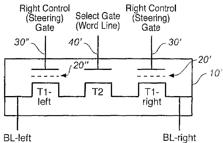
FIG. 1C (PRIOR ART)
