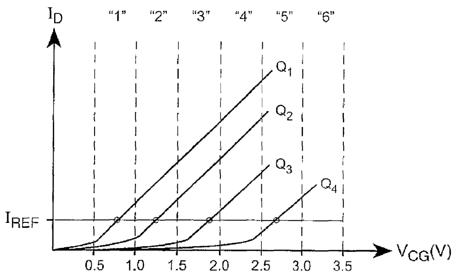
FIG. 4 (PRIOR ART)
