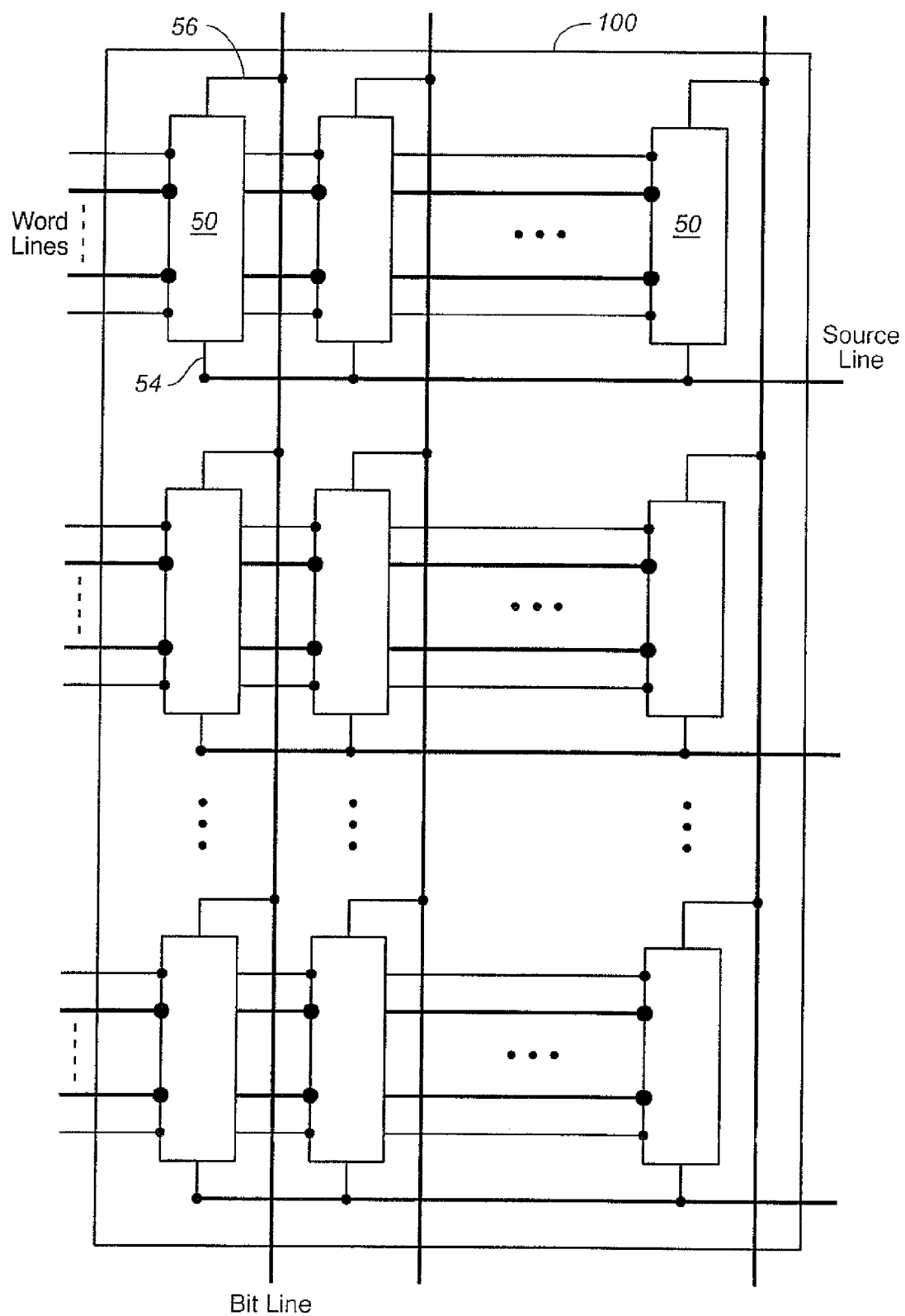
FIG. 3 (PRIOR ART)
