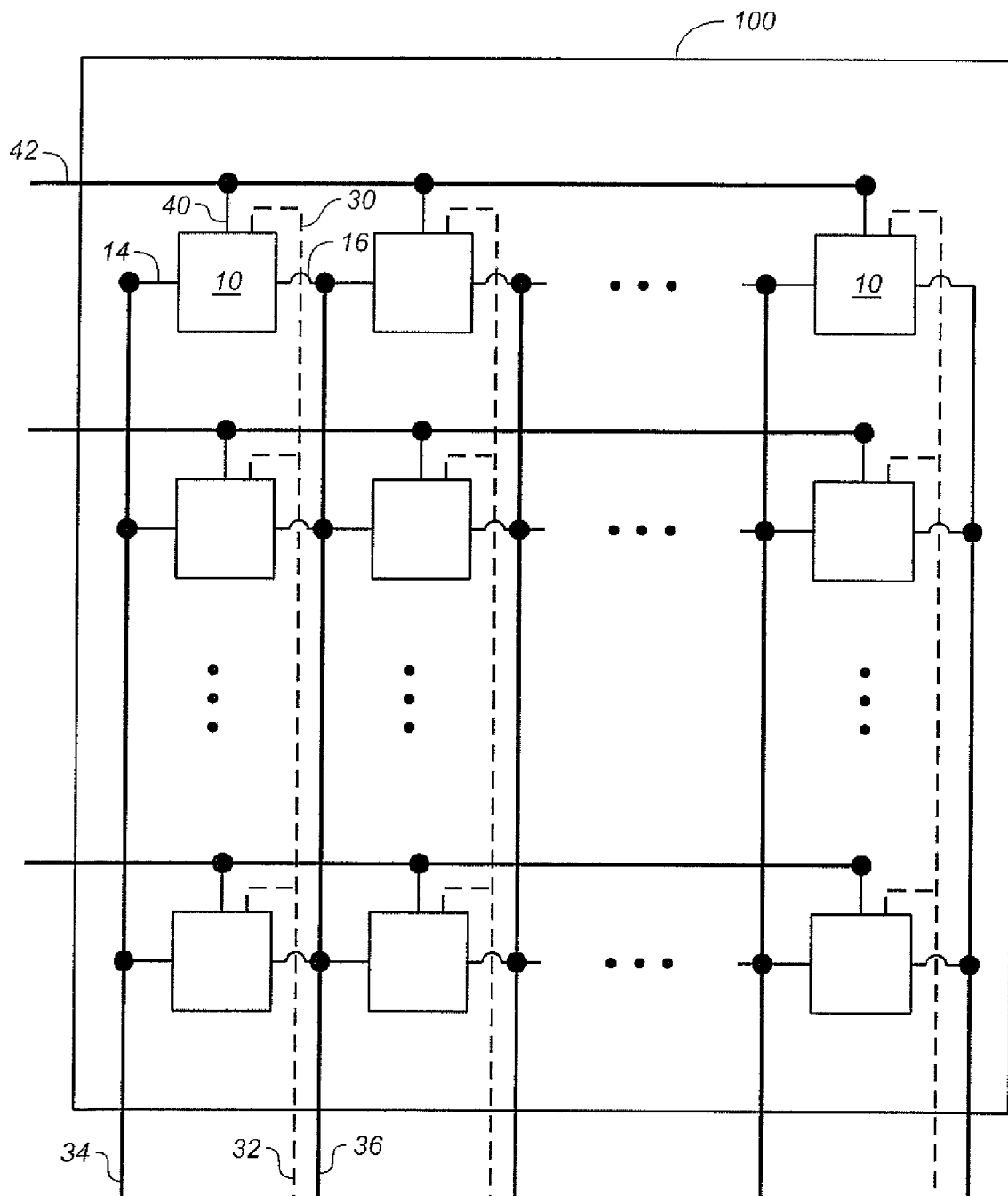
FIG. 2 (PRIOR ART)
