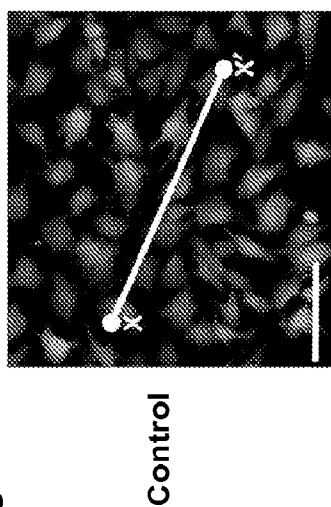
Fig. 3C1 Hs578T
