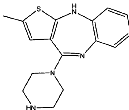
Metabolite B
