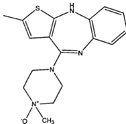
Metabolite A
