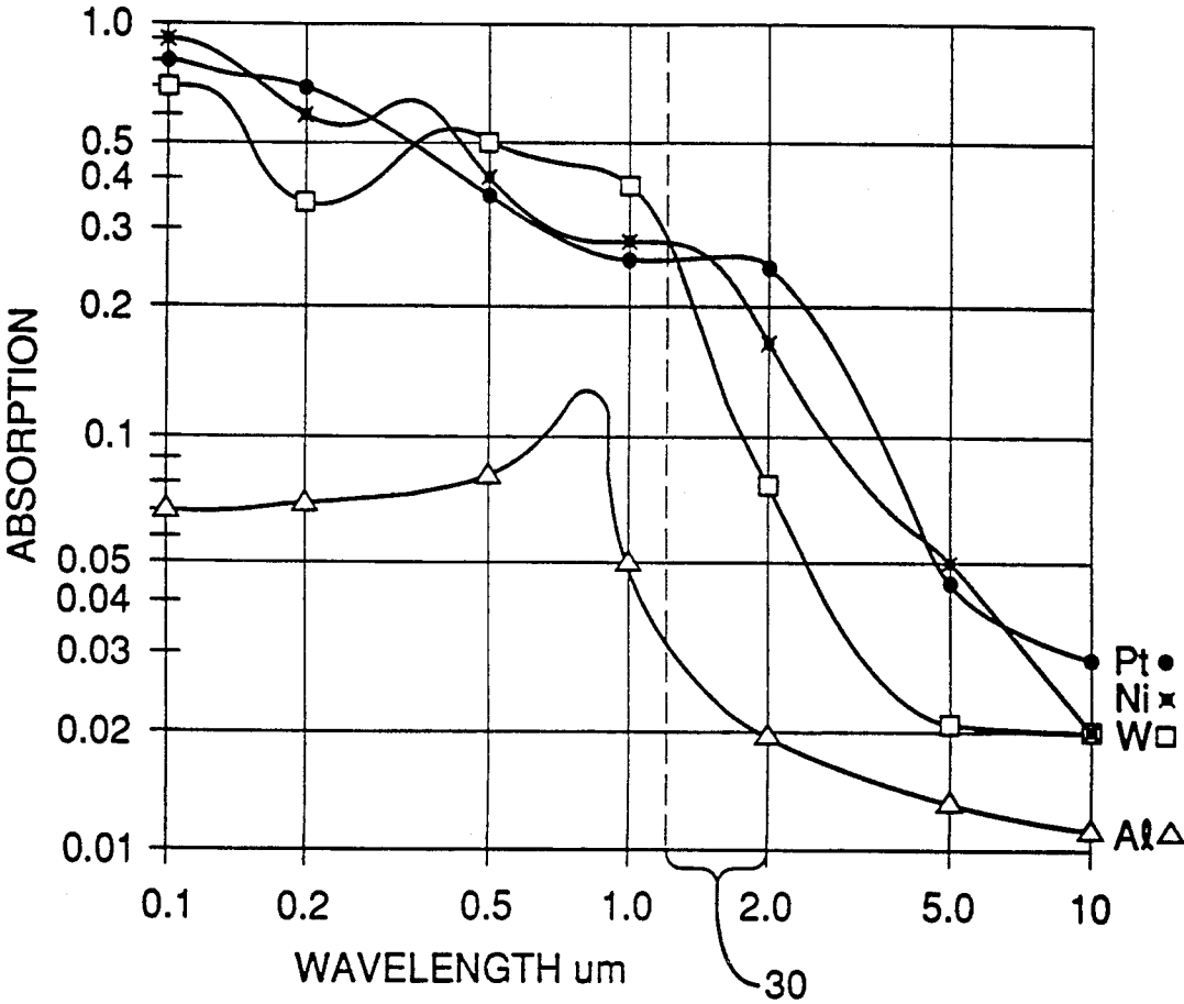
OPTICAL ENERGY ABSORPTION VS. WAVELENGTH FOR METALS
