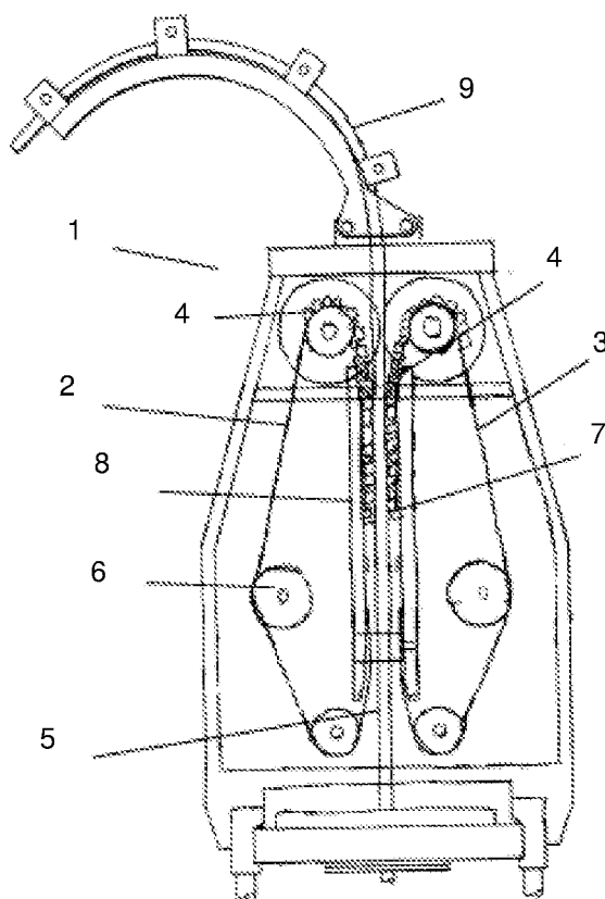
FIG. 1 PRIOR ART
